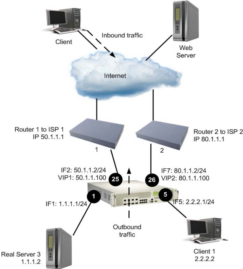
Figure 140: Simple WAN Link Load Balancing Example
