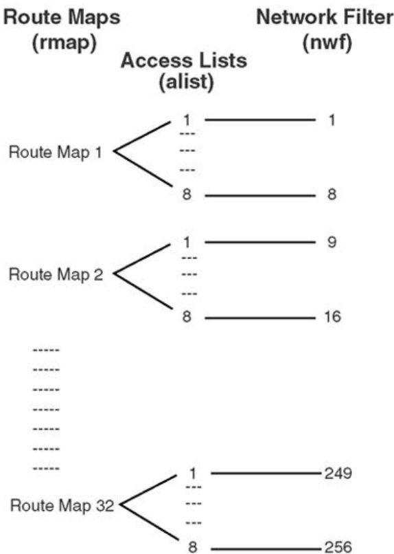
Figure 33: Relationship Between Route Maps, Access Lists, and Network Filters
