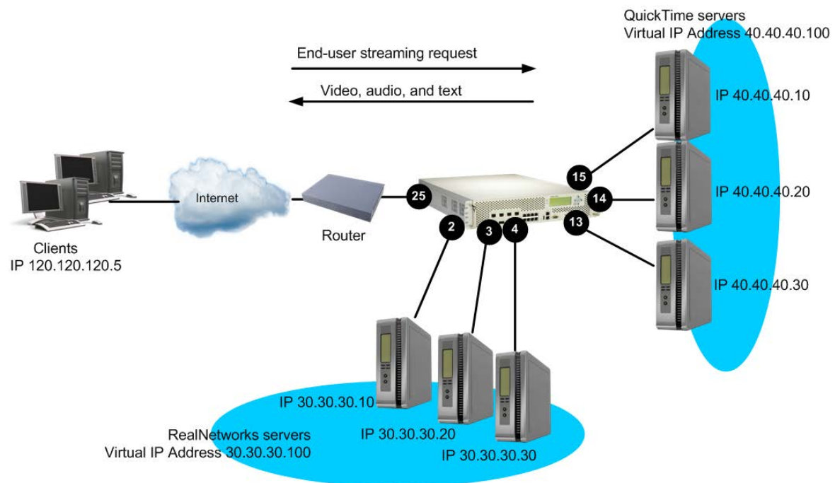
Figure 68: Load Balancing RTSP Servers
