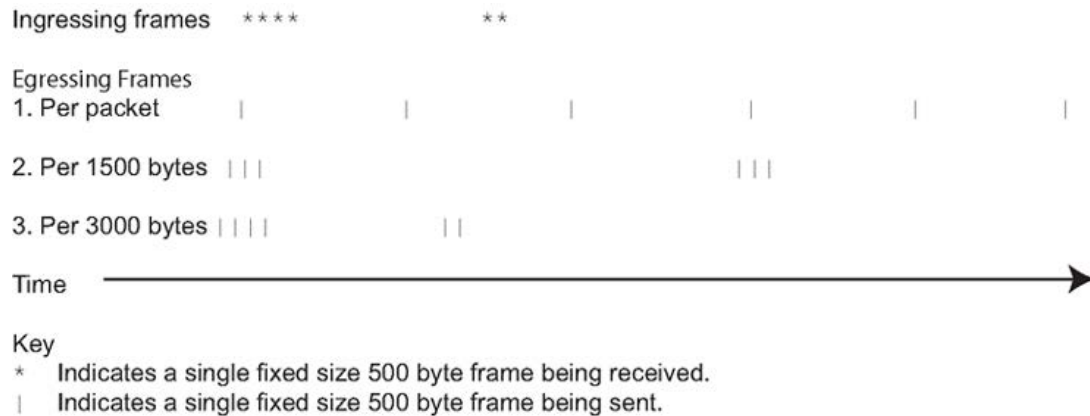
Figure 131: Real-time Clocks and Theoretical Departure Times
