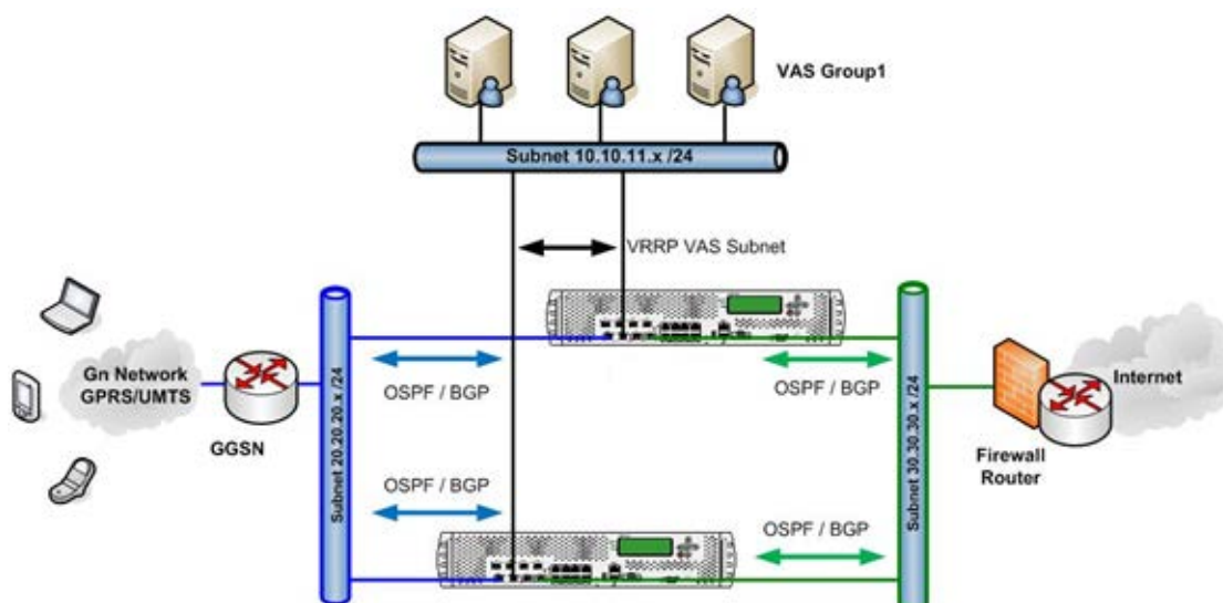
Figure 148: OSPF VRRP Topology Using Cost Updating
