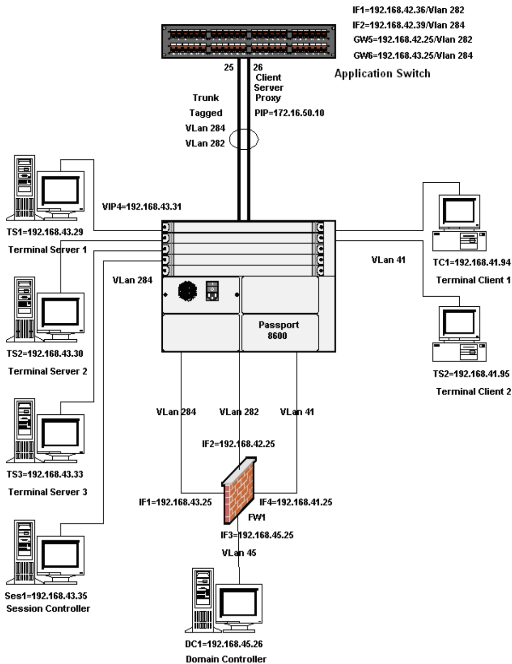
Figure 84: Windows Terminal Server Load Balancing Network Topology
