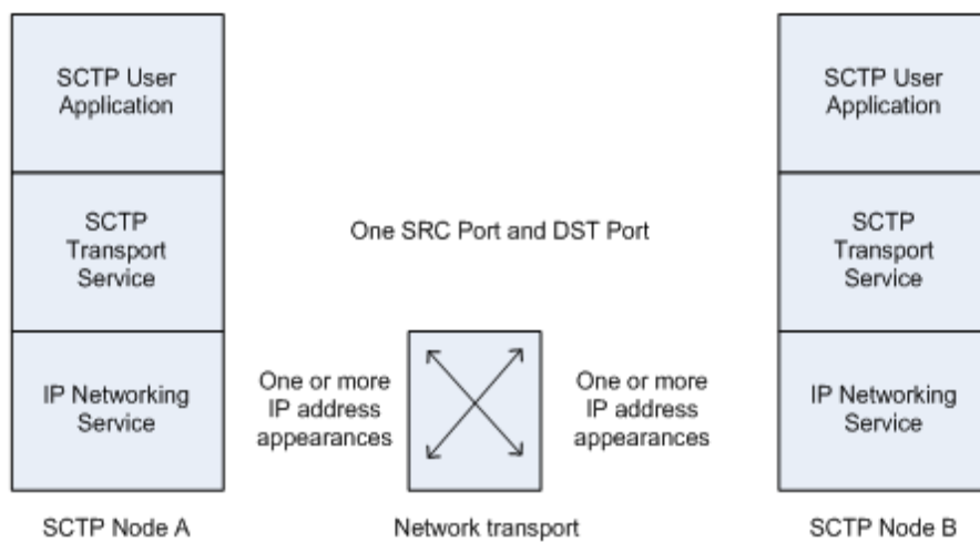
Figure 76: SCTP association concept diagram
