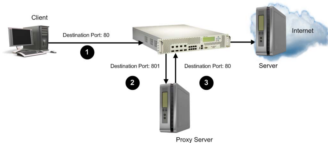
Figure 88: Redirecting Traffic with Port Address Translation
