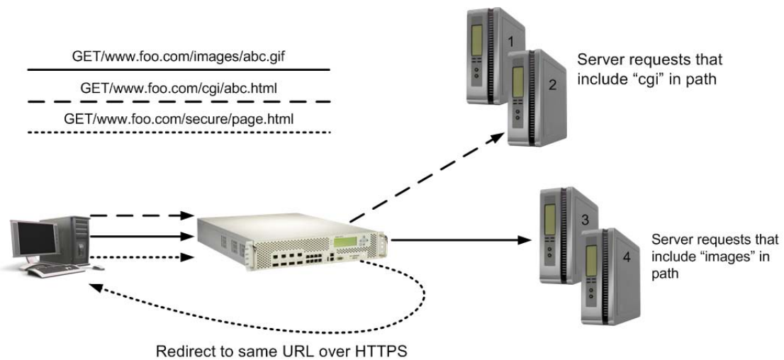
Figure 63: URL-Based SLB Scenario
