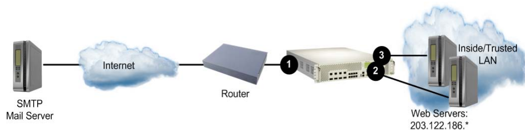
Figure 96: TCP Flag Filter Configuration Example
