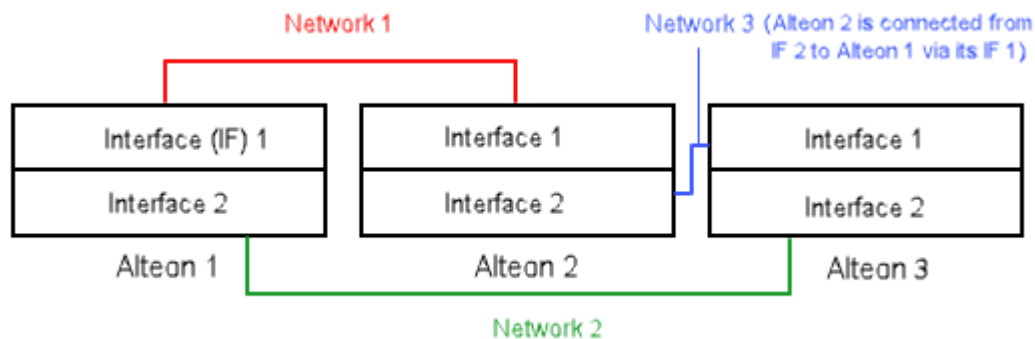
Figure 44: Example of Failback/Failover order configuration
