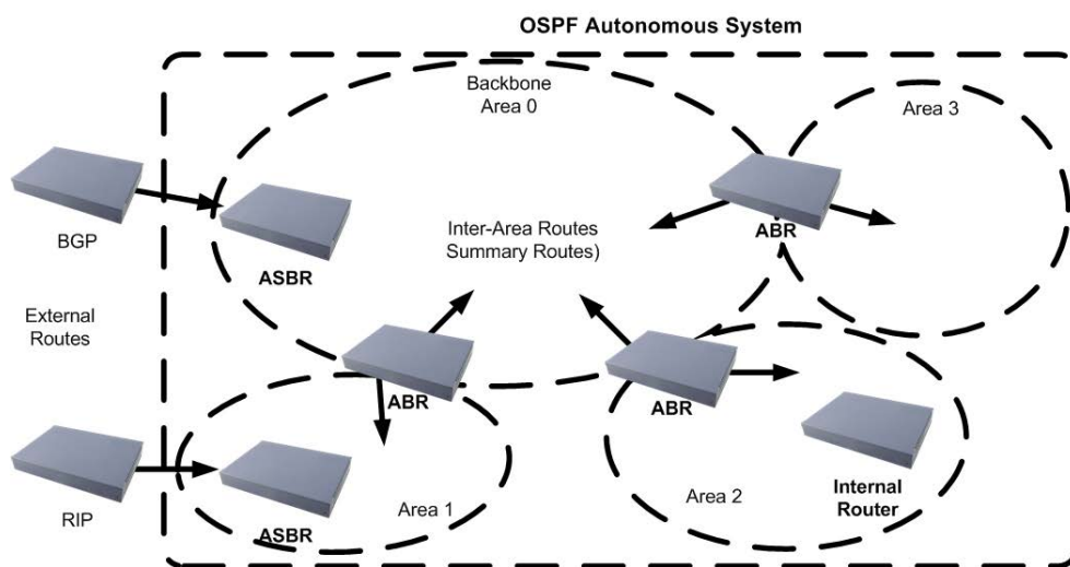
Figure 37: OSPF Routing Device Types
