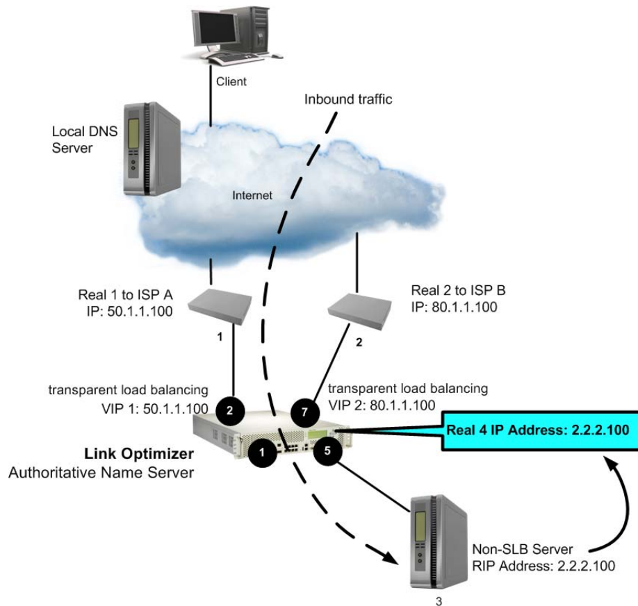
Figure 138: External Client Accessing Data from a Non-SLB Group
