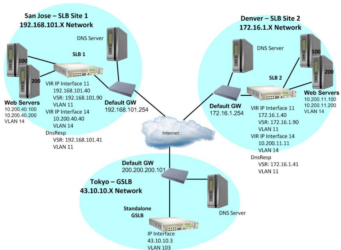
Figure 99: GSLB Topology with a Standalone GSLB Site Example
