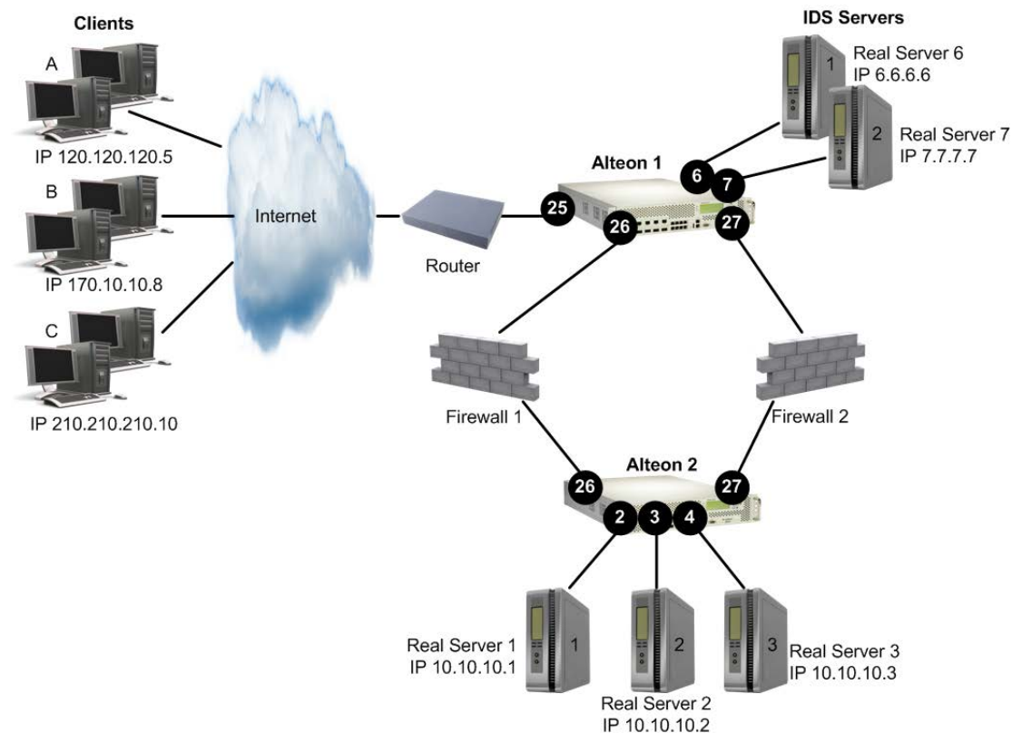
Figure 71: Server Load Balancing and IDS Load Balancing to a Single Group
