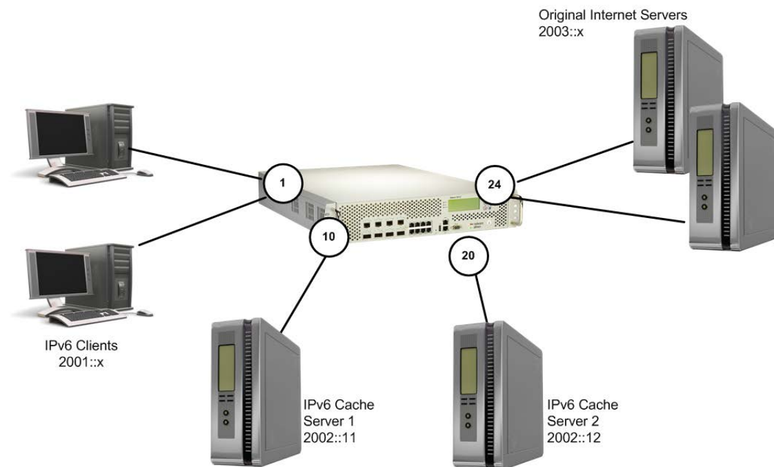
Figure 143: TCP Service Port Based HTTP Redirection
