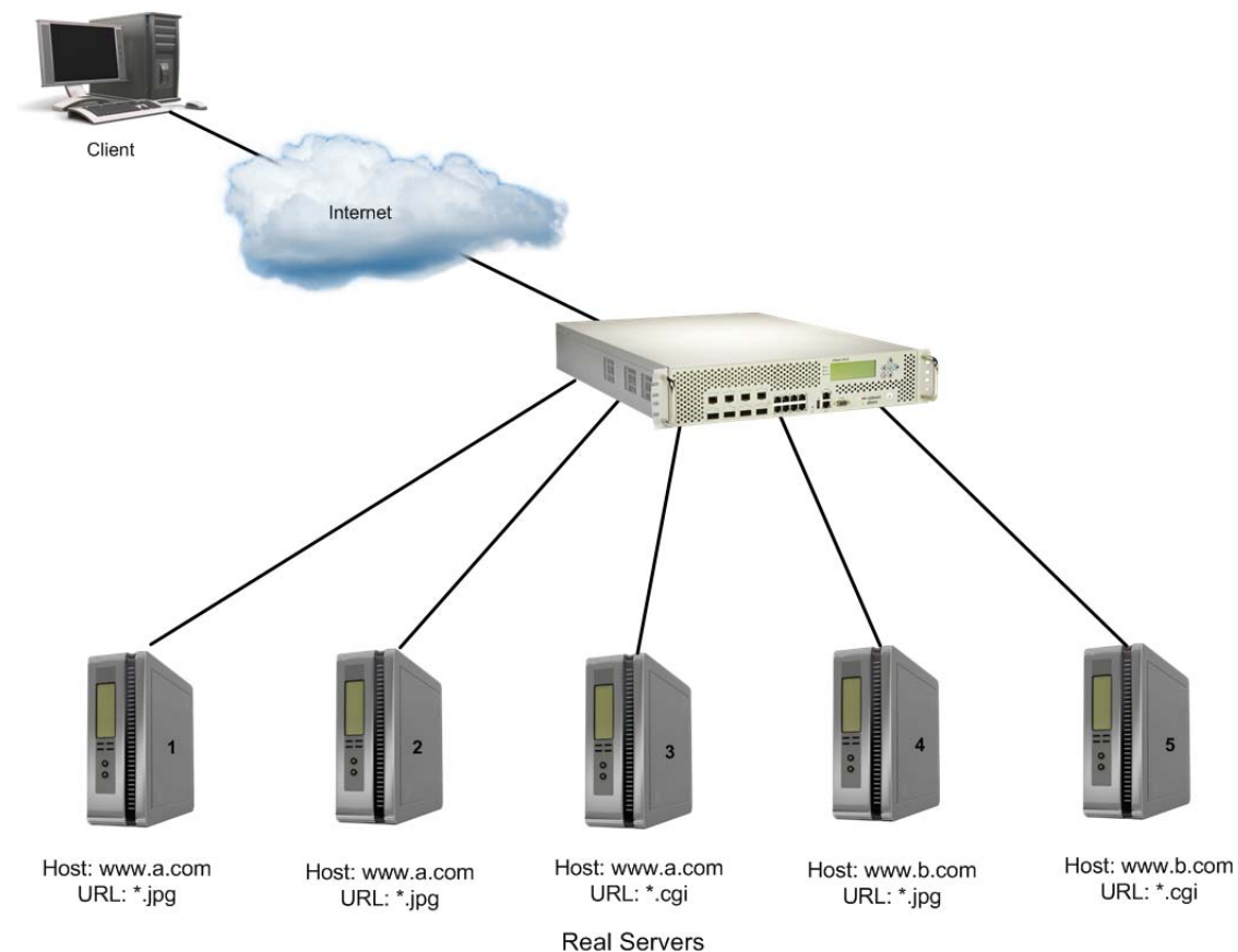
Figure 136: Content Precedence Lookup Multiple Strings Example
