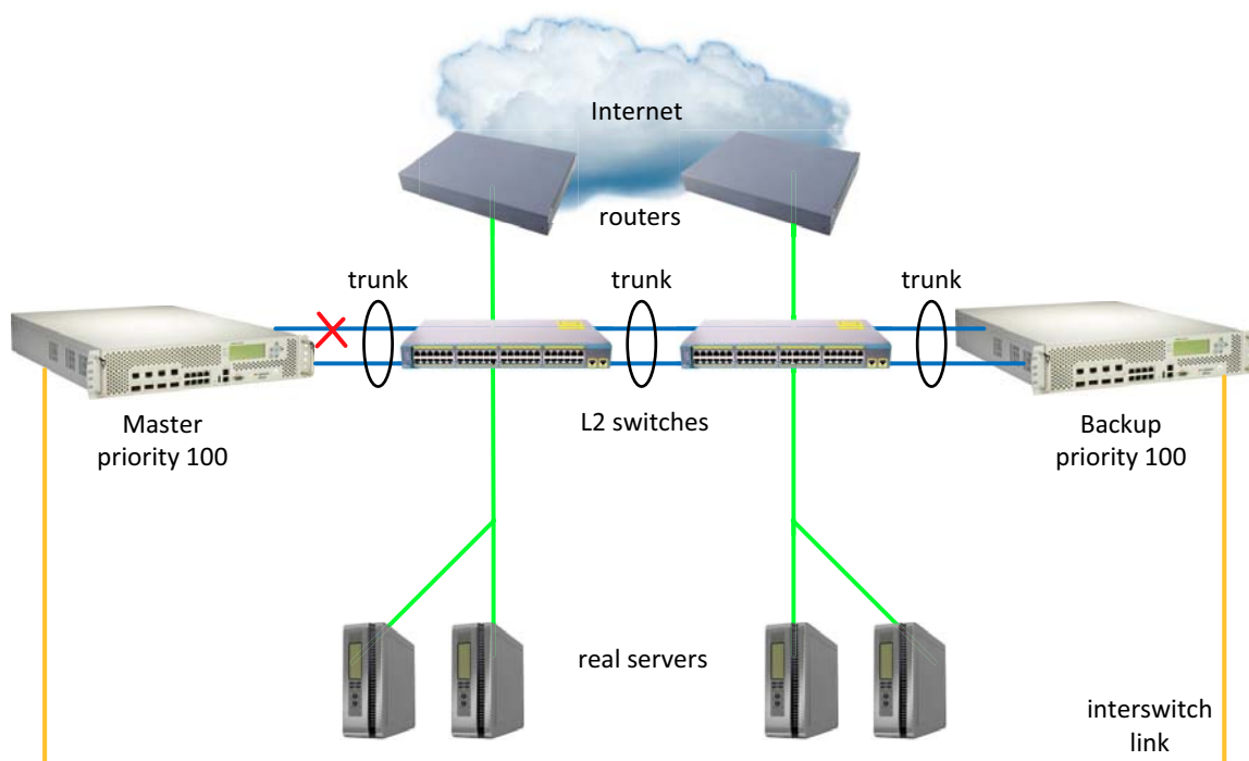
Figure 146: Trunk Port Failure
