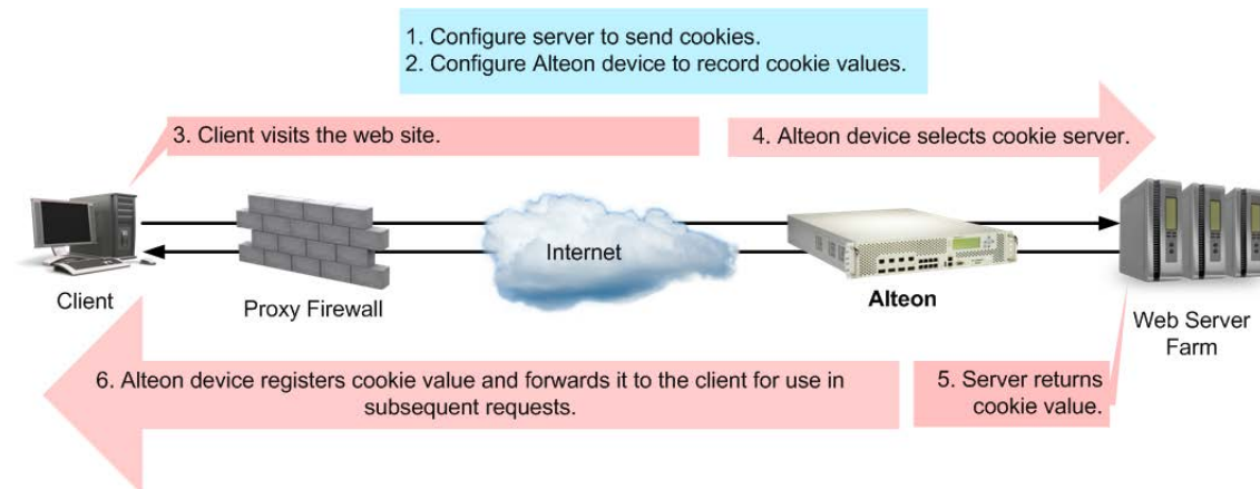
Figure 81: Passive Cookie Mode
