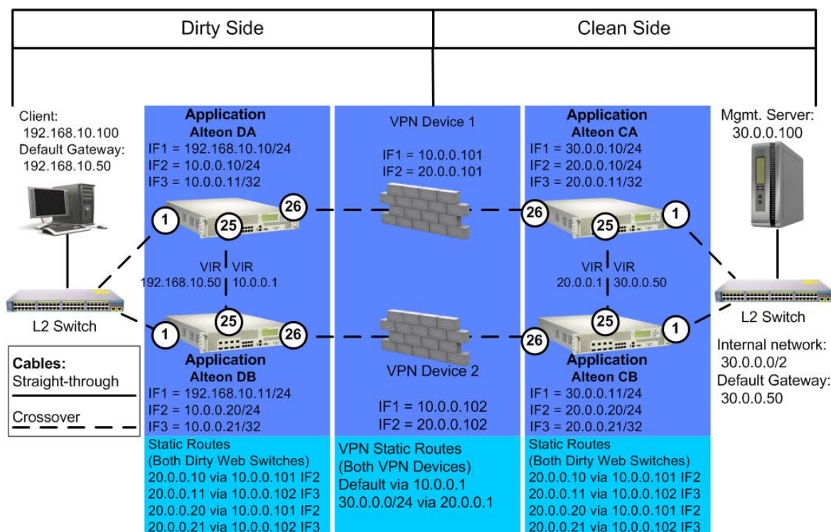
Figure 122: Example VPN Load Balancing Configuration
