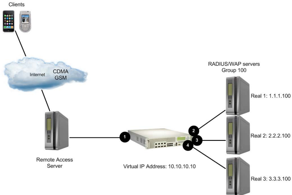
Figure 70: Load Balancing WAP Gateways
