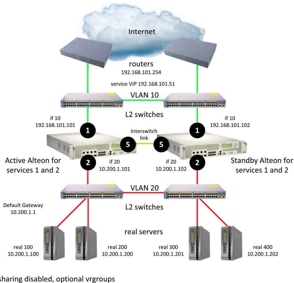
Figure 157: Session Mirroring
