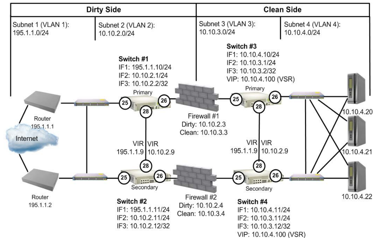
Figure 119: Four-Subnet Network
