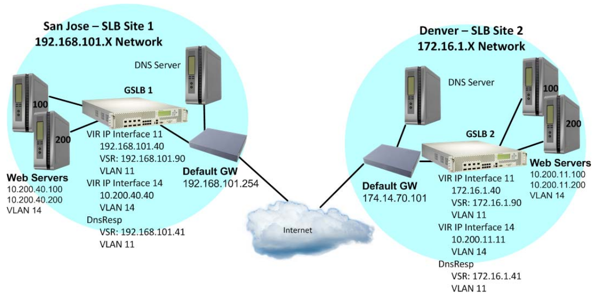
Figure 98: GSLB Topology Example
