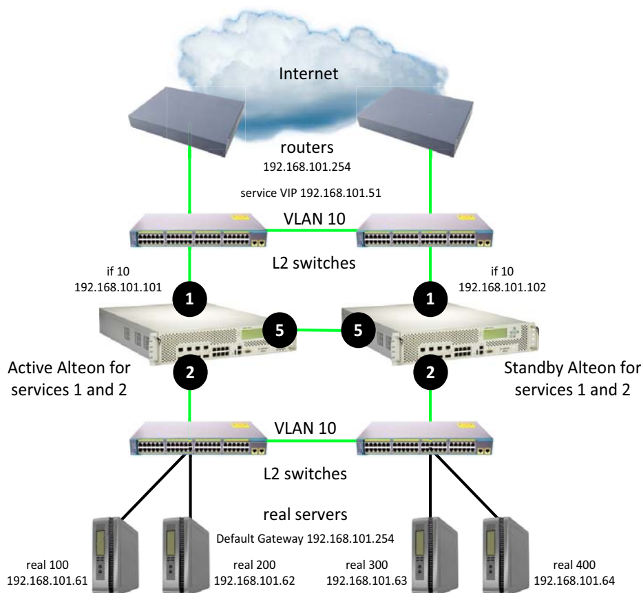
Figure 159: Single VLAN with Layer 2 Loops (Hot-Standby)
