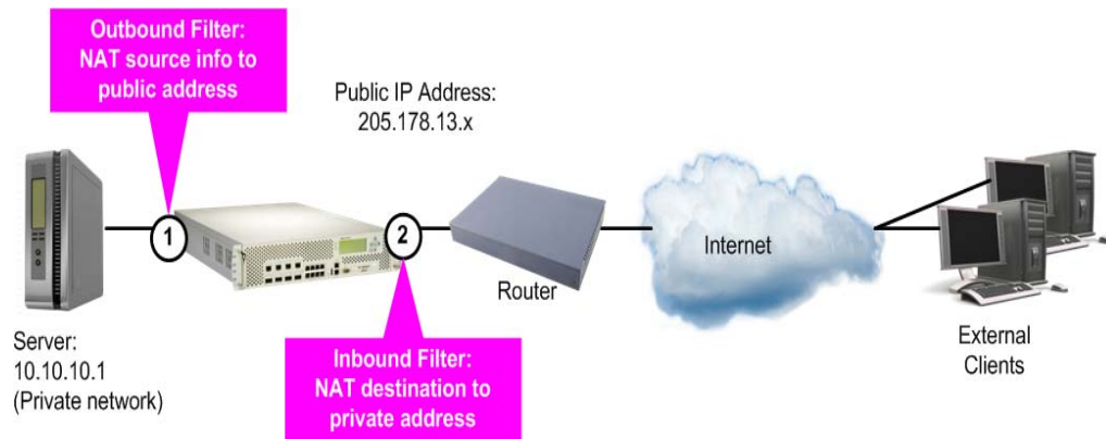
Figure 93: Static NAT Example
