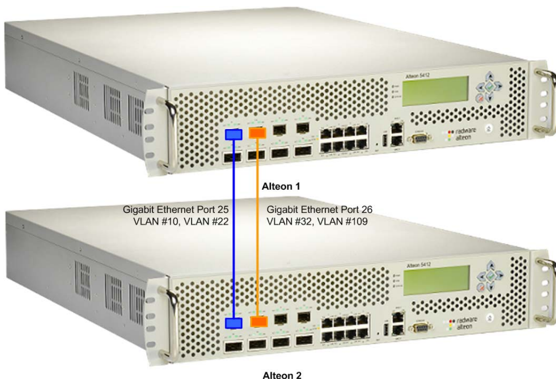
Figure 22: Parallel Links with VLANs Example
