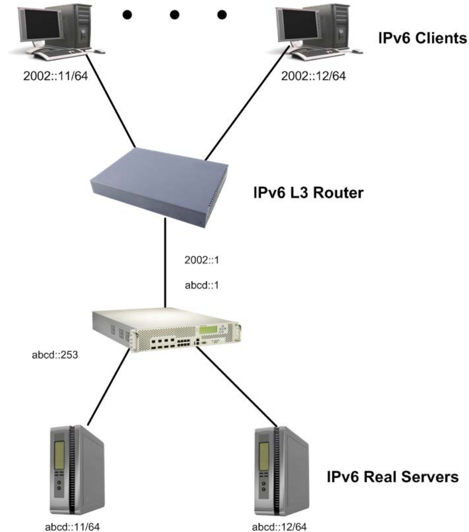
Figure 62: IPv6 to IPv6 Layer 4 SLB Example
