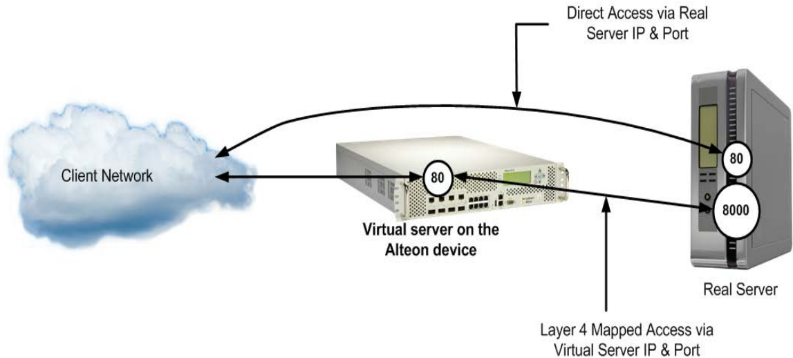
Figure 58: Mapped and Non-Mapped Server Access
