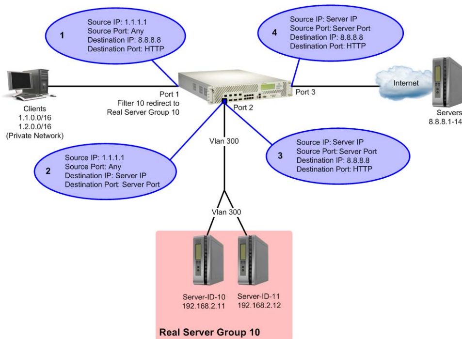
Figure 90: Redirecting Traffic with a Non-Transparent Server
