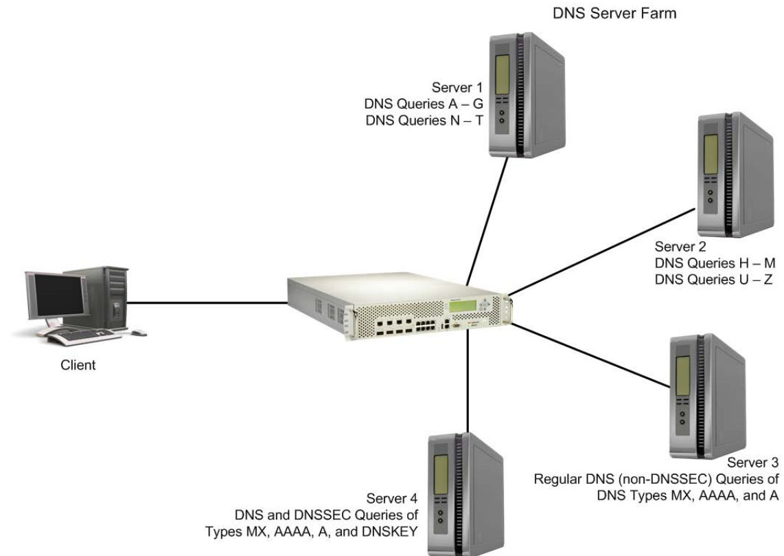
Figure 166: Load Balancing DNS Queries
