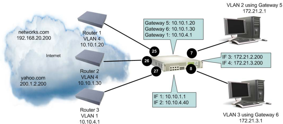
Figure 23: Example Segregation of VLAN Traffic Configuration
