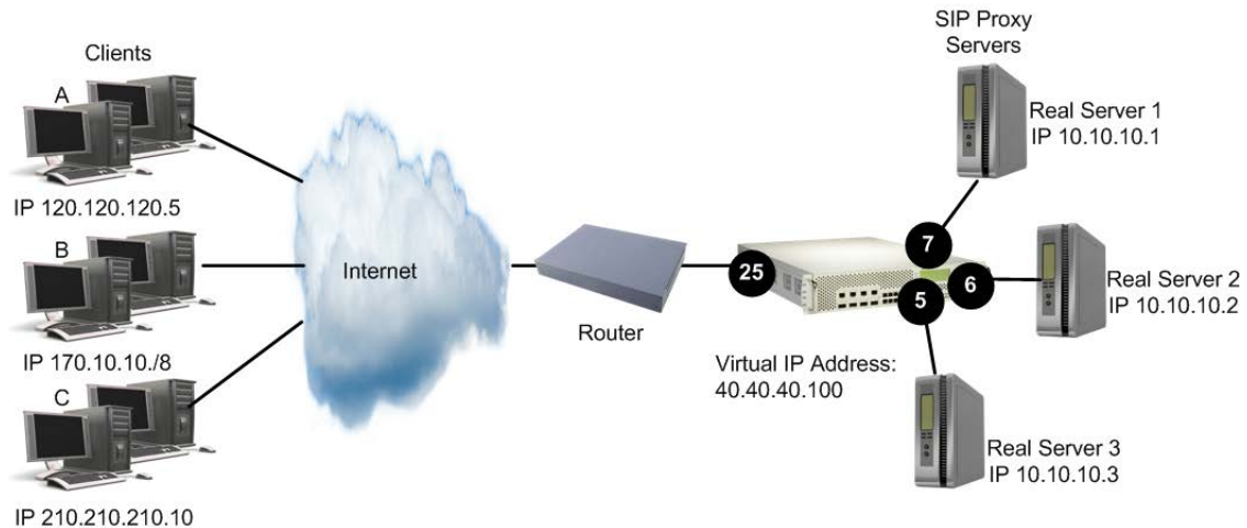
Figure 75: SIP Load Balancing Configuration Example
