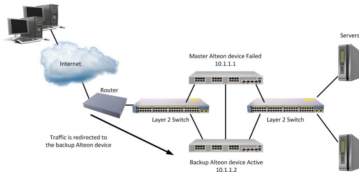
Figure 45: Stateful Failover Example when the Primary Alteon Fails
