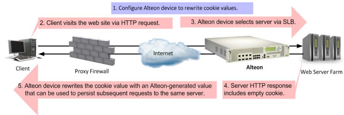
Figure 82: Rewrite Cookie Mode
