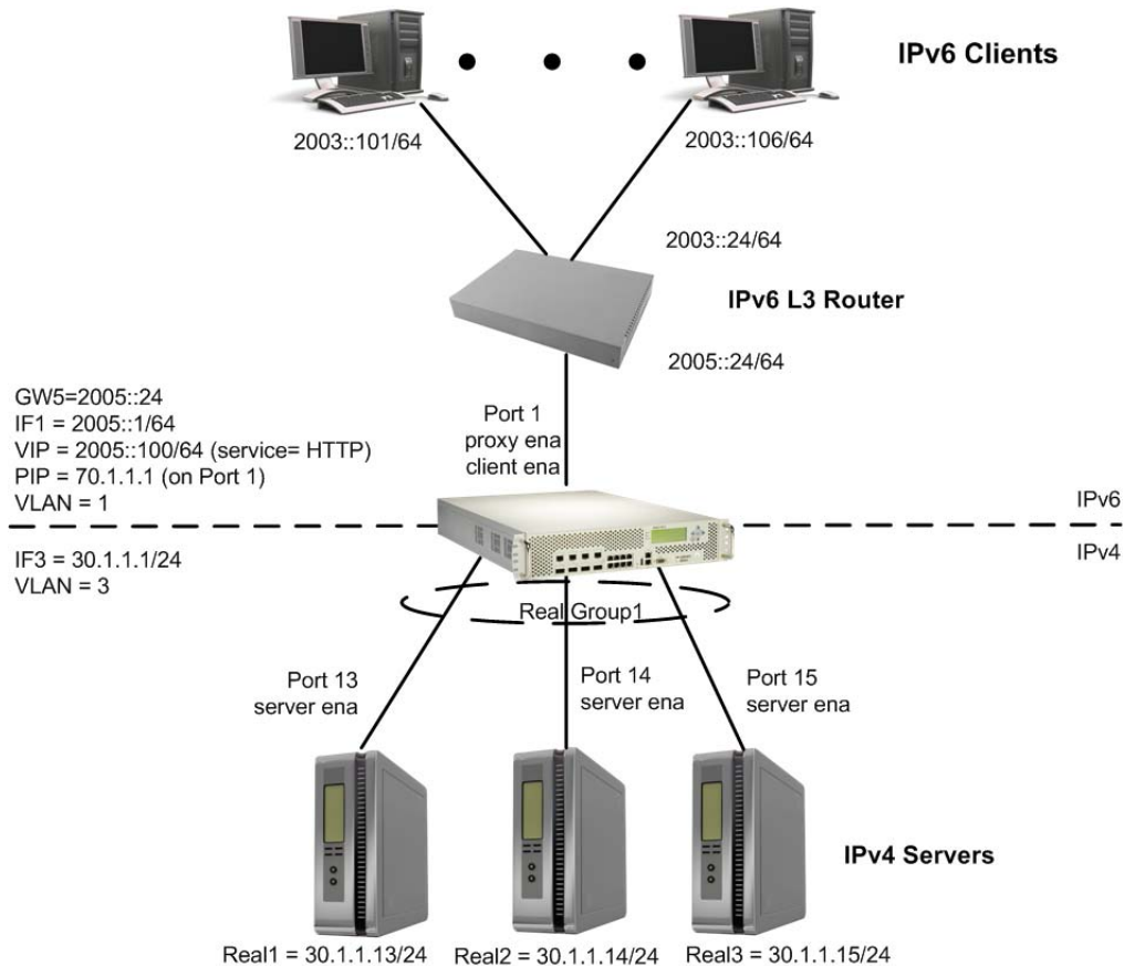
Figure 61: IPv6 to IPv4 Layer 4 SLB Example
