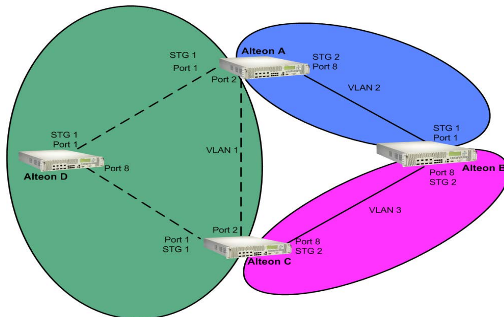
Figure 28: Four-Alteon Topology with a Multiple Spanning Tree
