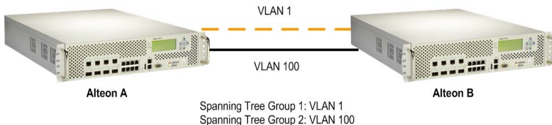
Figure 26: Example Multiple Spanning Tree Configuration
