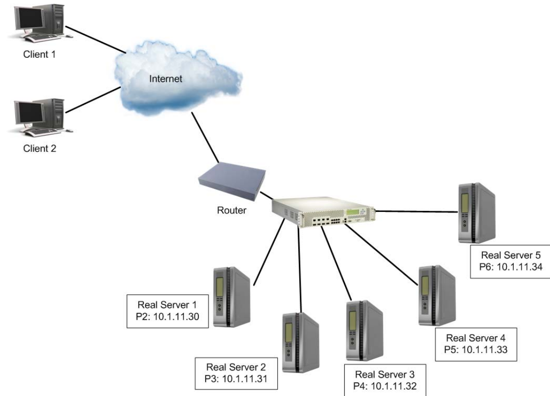
Figure 54: Example Buddy Server Health Check Configuration
