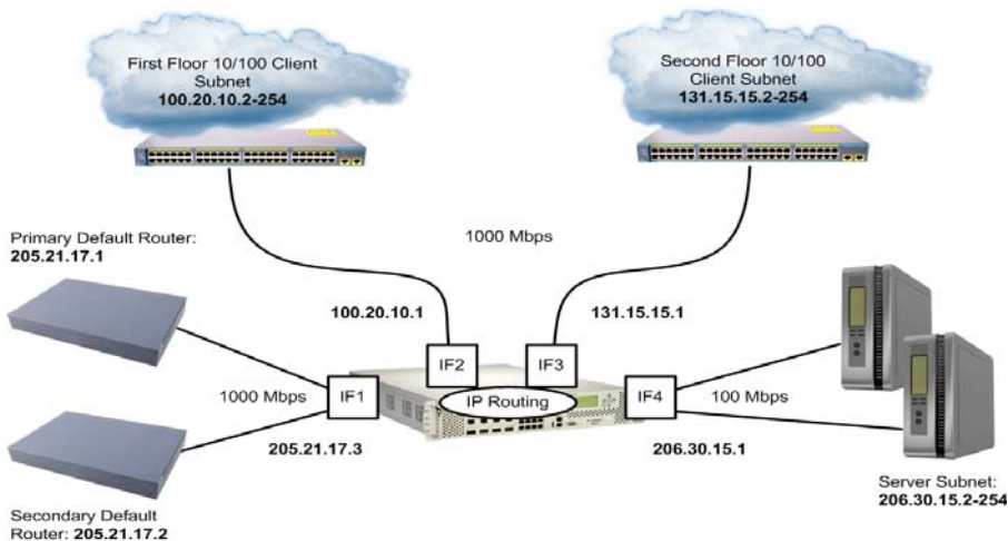
Figure 30: Example Configuration IP Subnet Routing with Alteon
