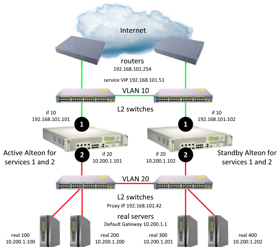
Figure 154: Separate Client and Server Ports with a Single Service, with PIP
