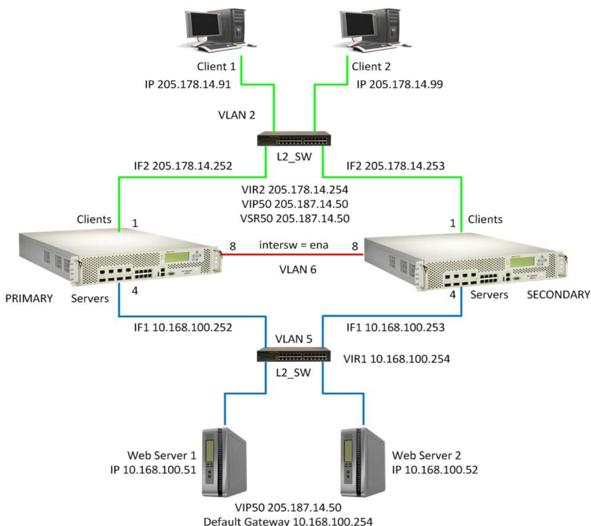
Figure 150: Active-Standby Session Mirroring
