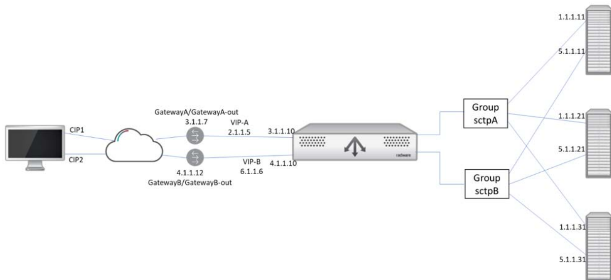
Figure 77: Example of multi-homed Sctp (N=M=2)
