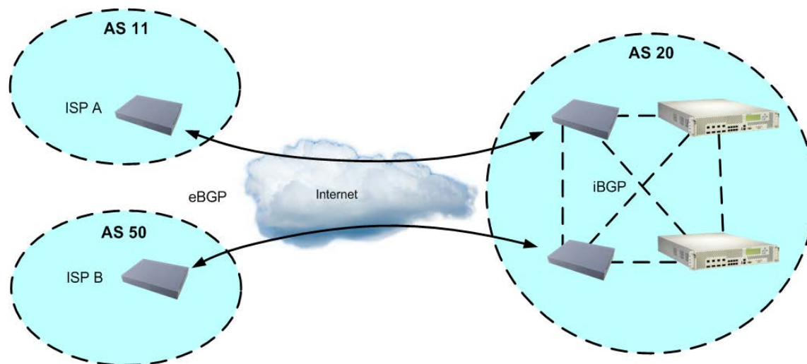
Figure 32: Example Topology using the Border Gateway Protocol (BGP)
