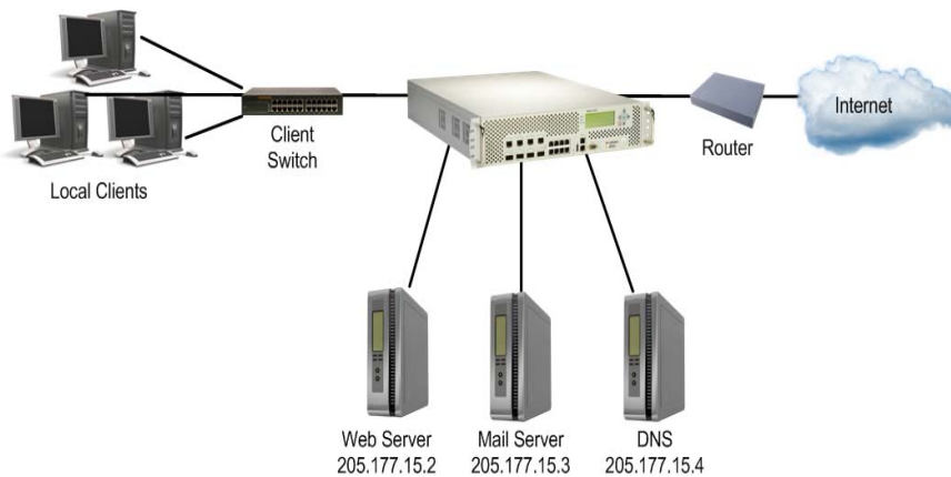
Figure 92: Filter-Based Security Configuration Example
