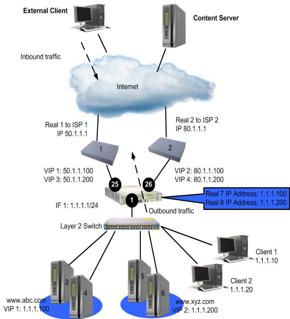
Figure 141: WAN Link Load Balancing with Server Load Balancing
