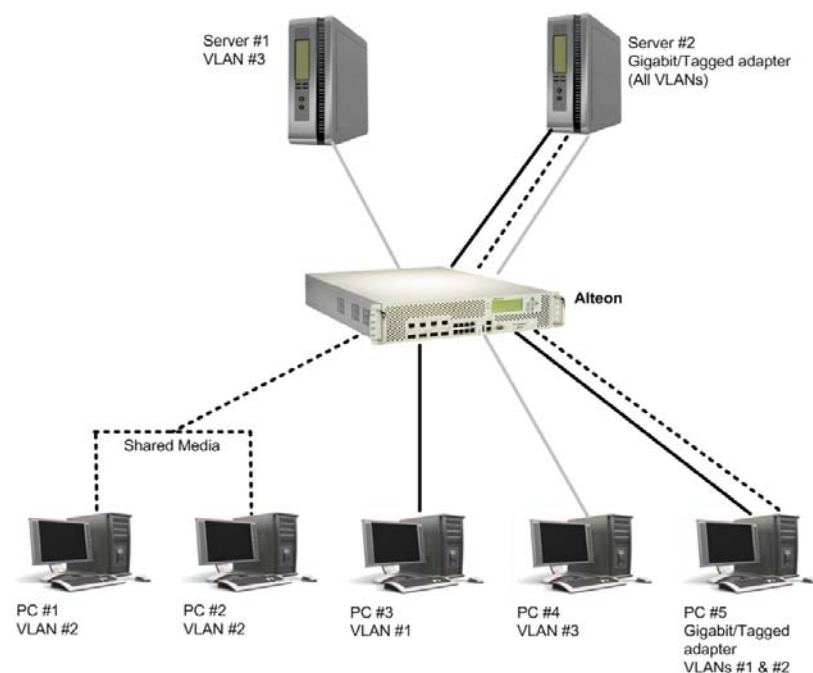
Figure 21: Multiple VLANs with Tagging Adapters Example
