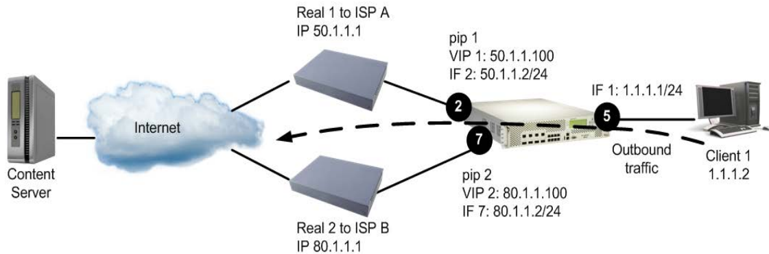
Figure 137: WAN Link Load Balancing for Outbound Traffic
