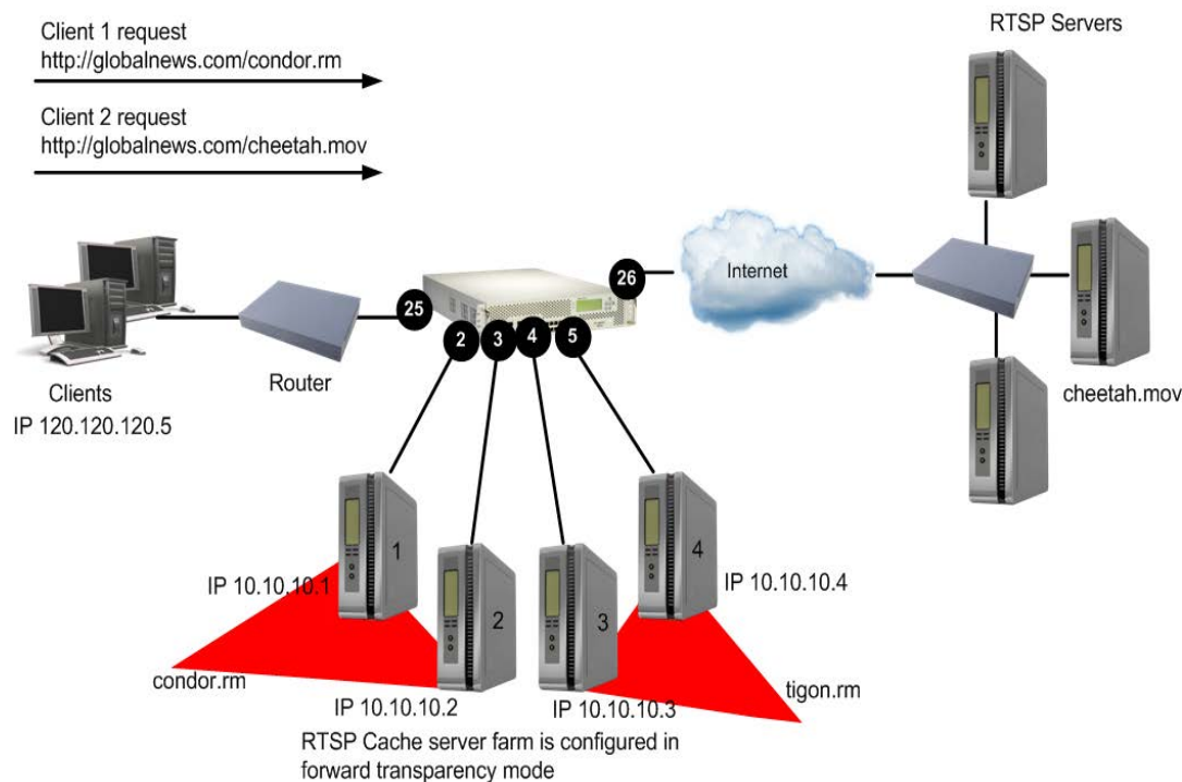
Figure 110: RTSP Streaming Cache Redirection
