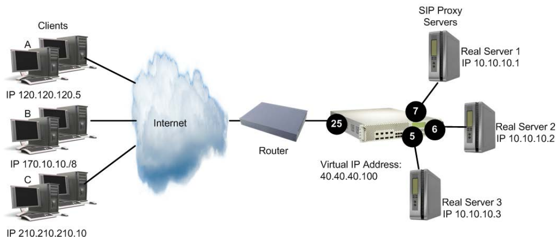
Figure 74: SIP Load Balancing
