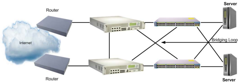
Figure 162: Loops in an Active-Active Configuration
