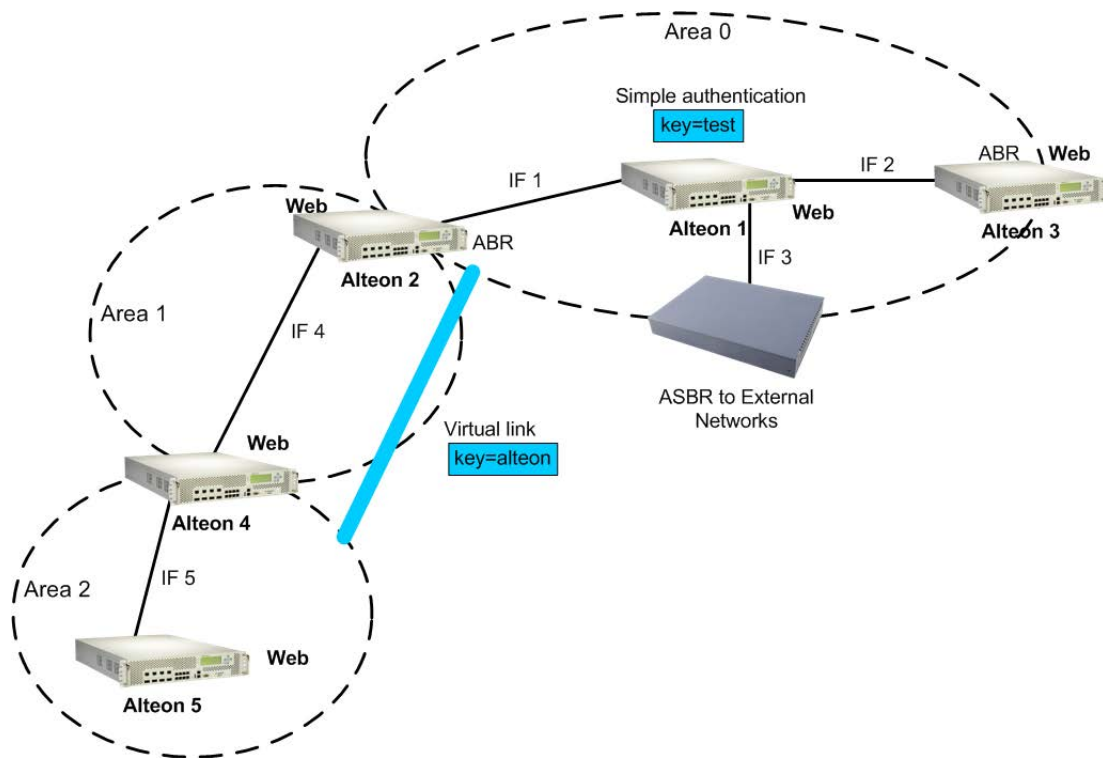
Figure 39: Authentication Example
