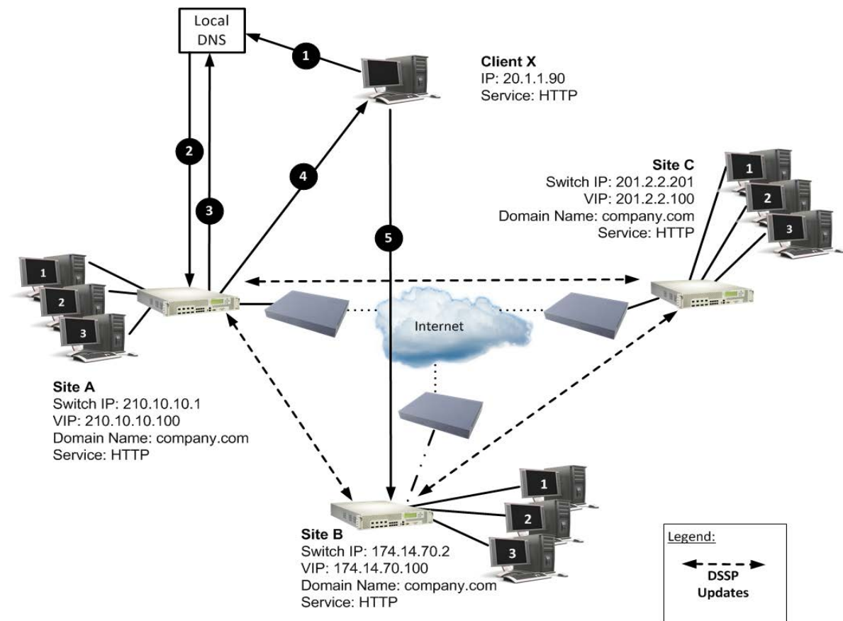
Figure 100: GSLB Client Proximity Site with HTTP Service
