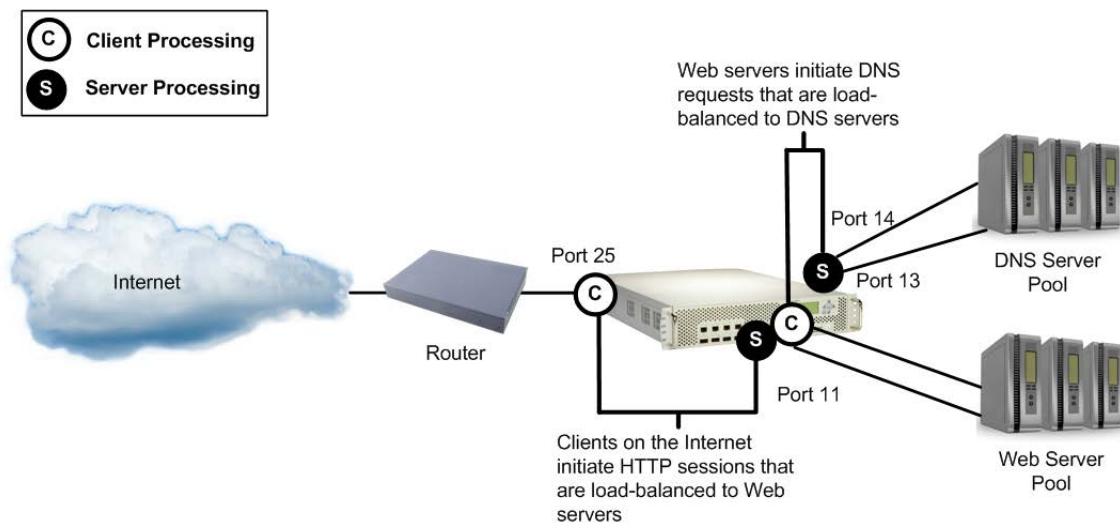
Figure 53: Example Network for Client/Server Port Configuration
