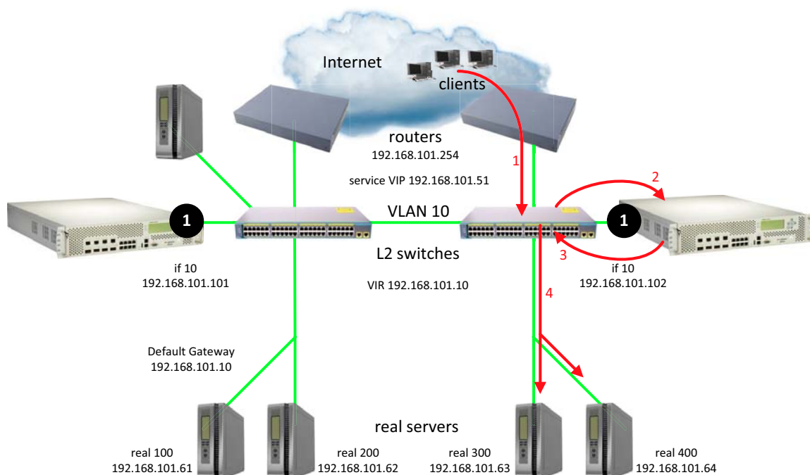
Figure 160: Single VLAN with Single IP Subnet in One Leg
