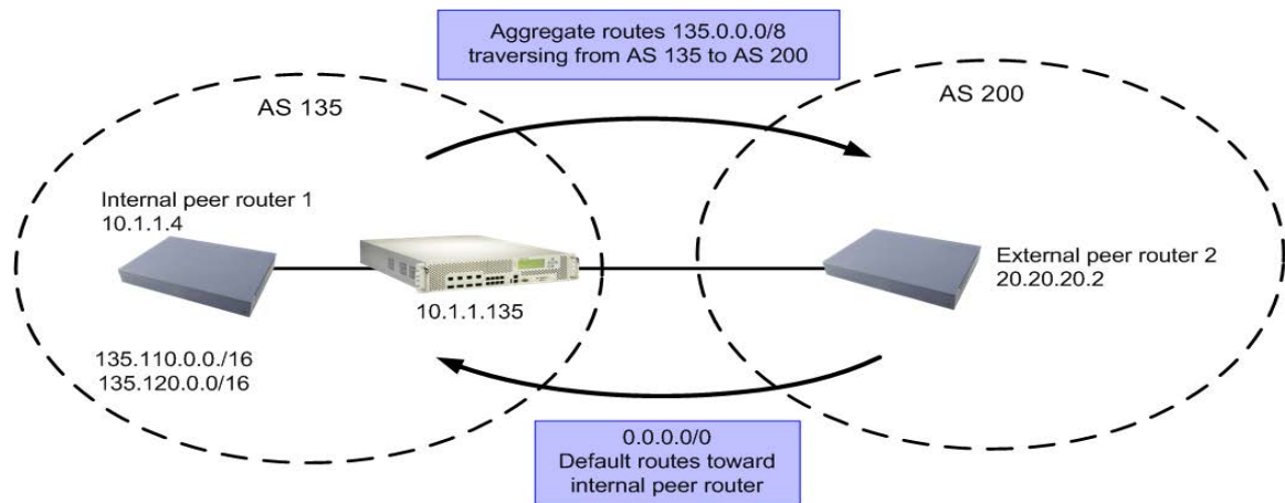
Figure 35: Default Redistribution and Route Aggregation Example
