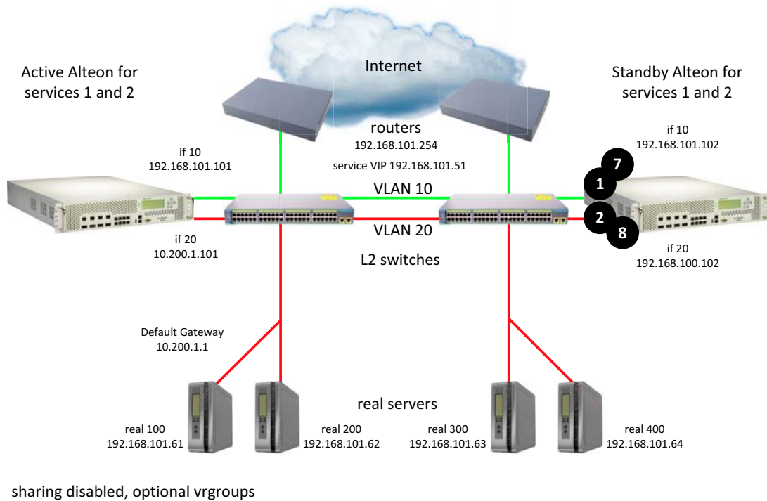
Figure 156: One-leg Design with LACP, no PIP
