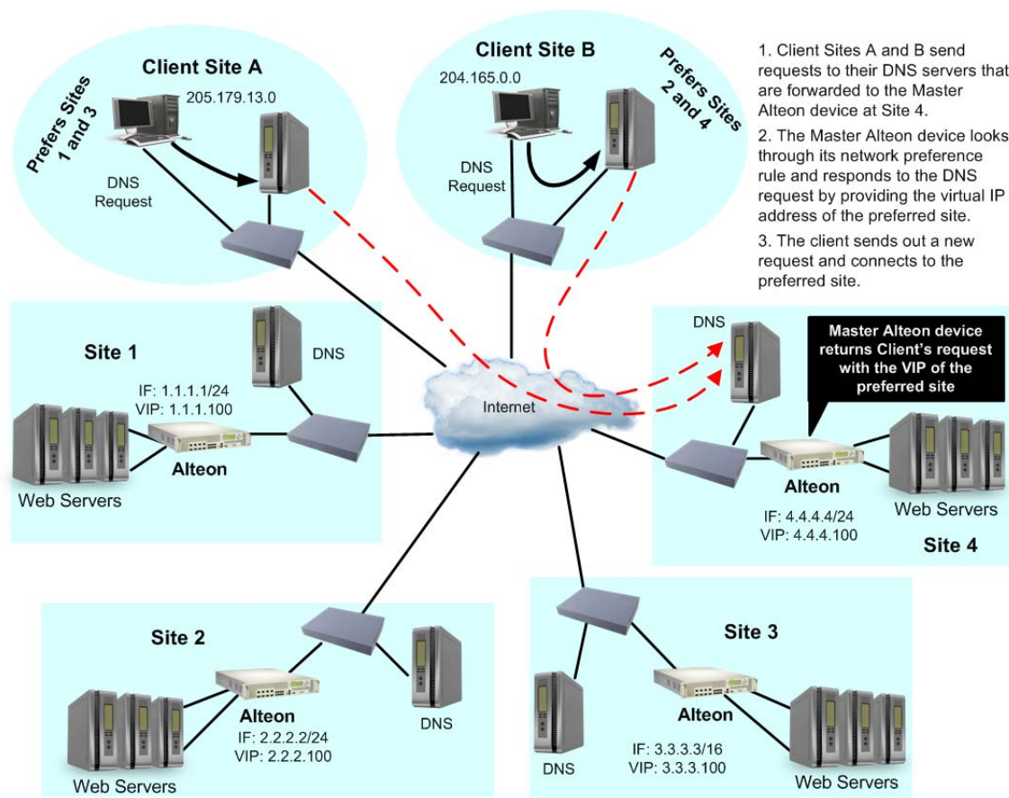
Figure 101: Configuring GSLB Network Preference
