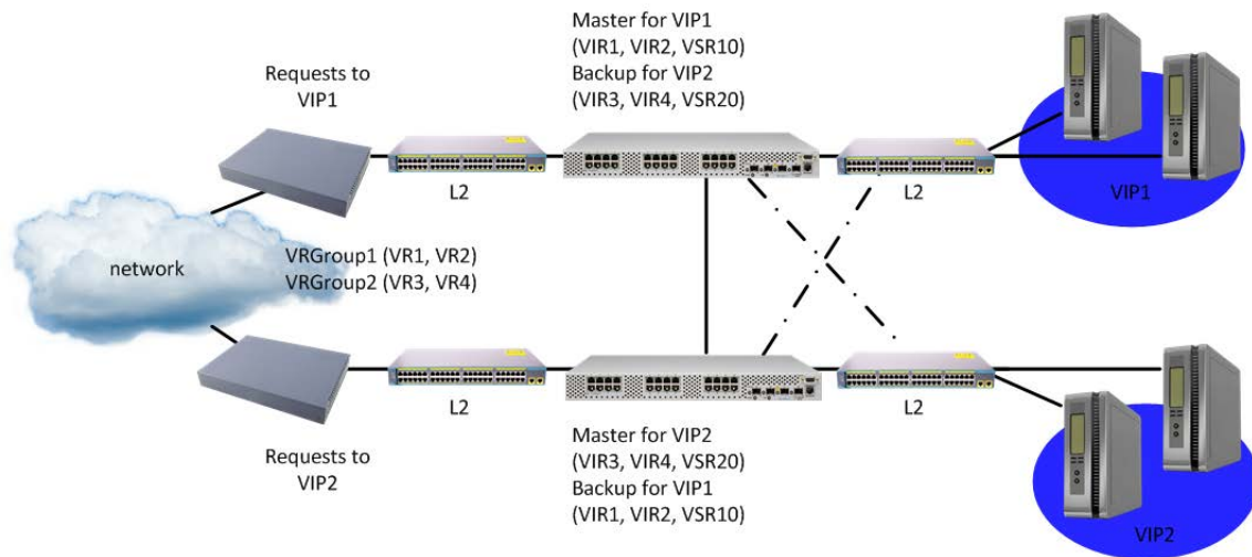
Figure 149: Service-based Virtual Router Groups in an Active-Standby Configuration
