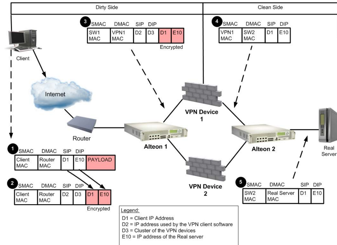
Figure 121: Basic Frame Flow
