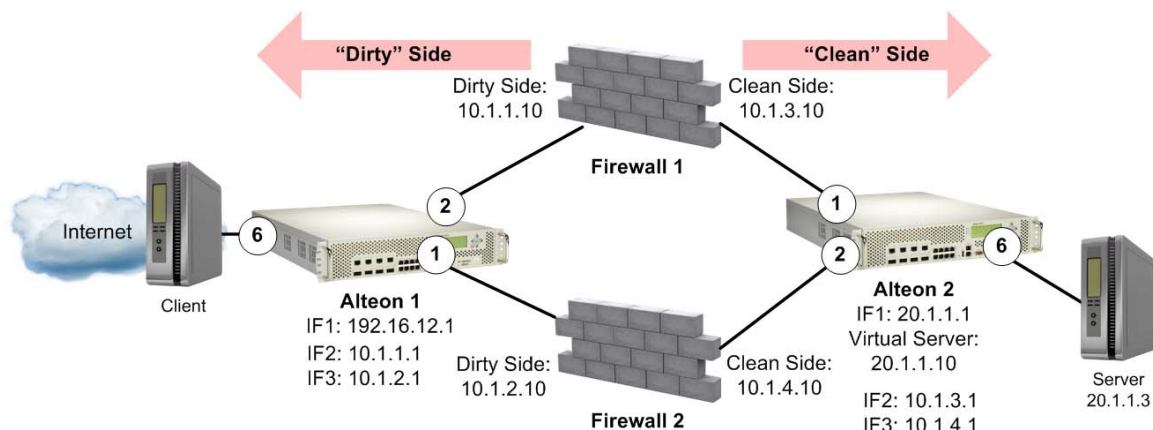
Figure 118: Basic FWLB Network
