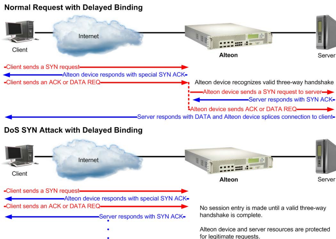
Figure 60: Normal Request with Delayed Binding
