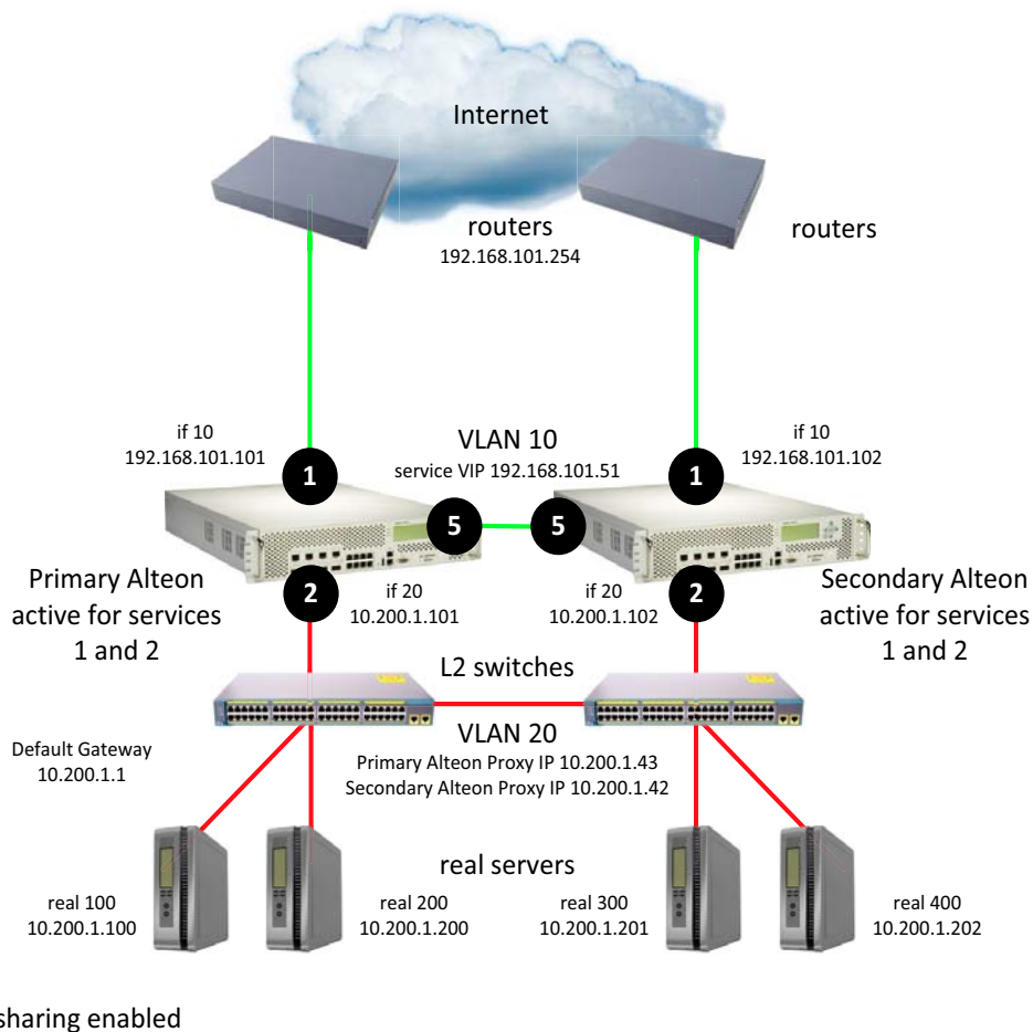
Figure 158: Multiple VLANs with Directly Attached Routers (Active-Active)
