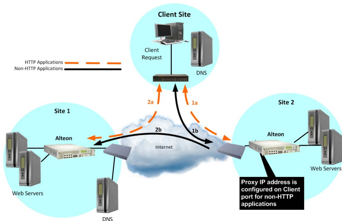
Figure 102: HTTP and Non-HTTP Redirects
