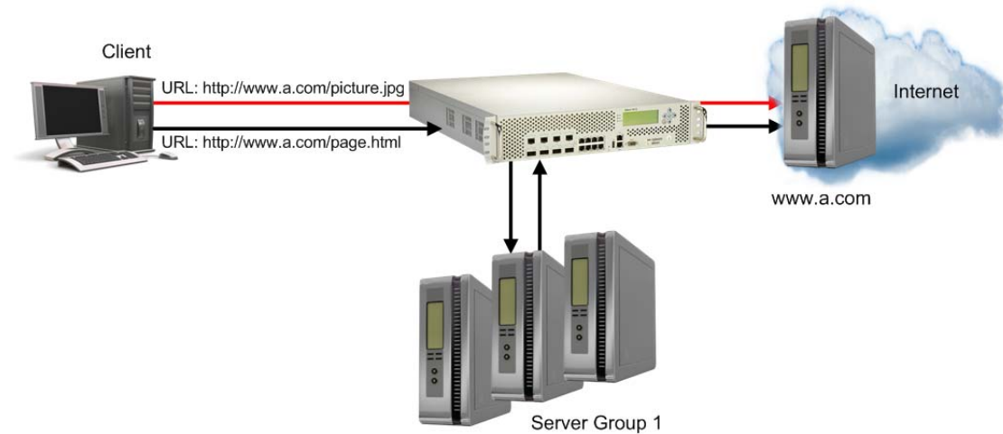
Figure 86: Redirecting Layer 7 Traffic with a Transparent Server
