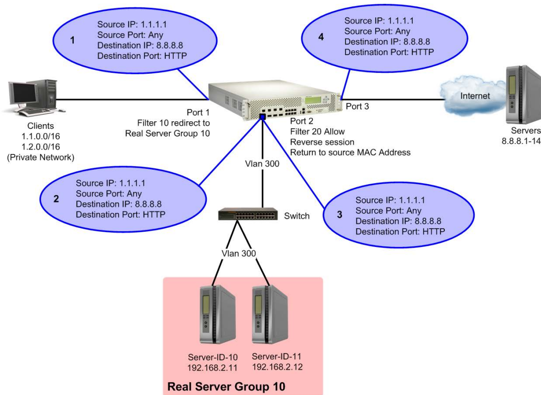
Figure 85: Redirecting Layer 4 Traffic with a Transparent Server
