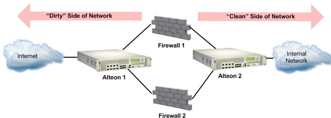
Figure 112: Basic FWLB Topology
