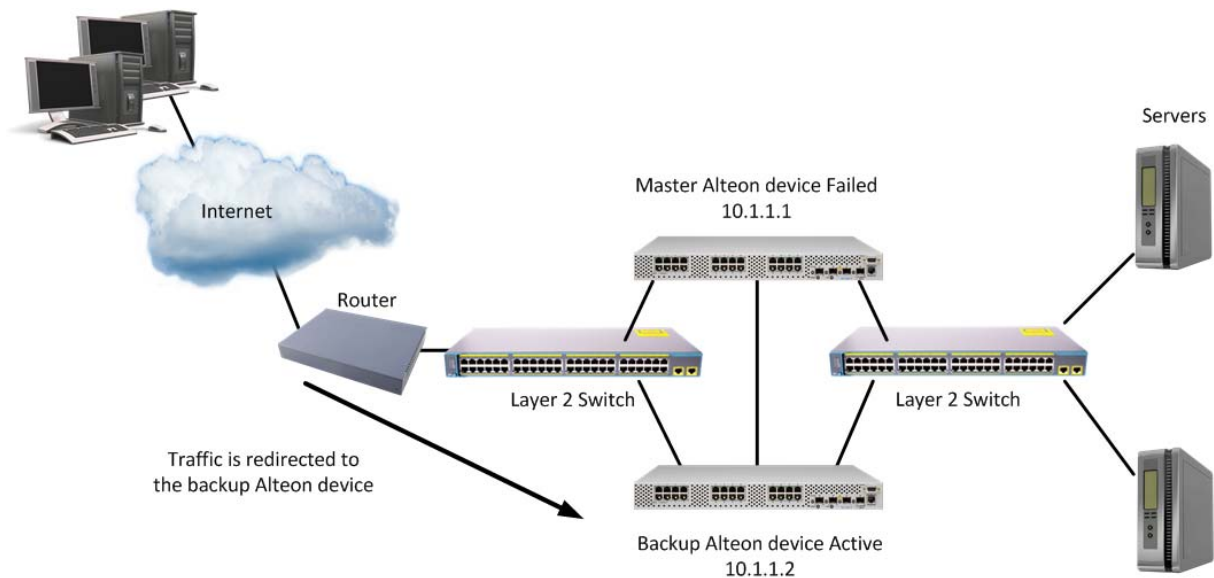
Figure 151: Stateful Failover Example when the Primary Alteon Fails
