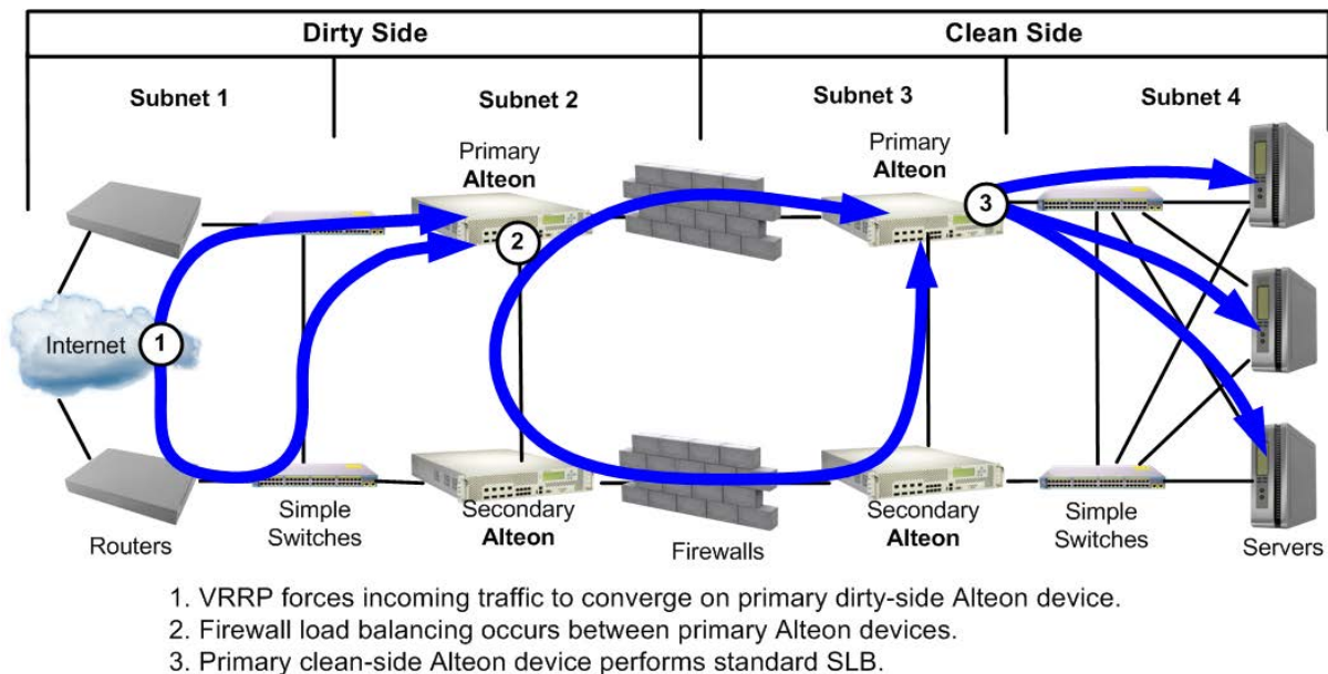
Figure 116: Example Four-Subnet FWLB Implementation
