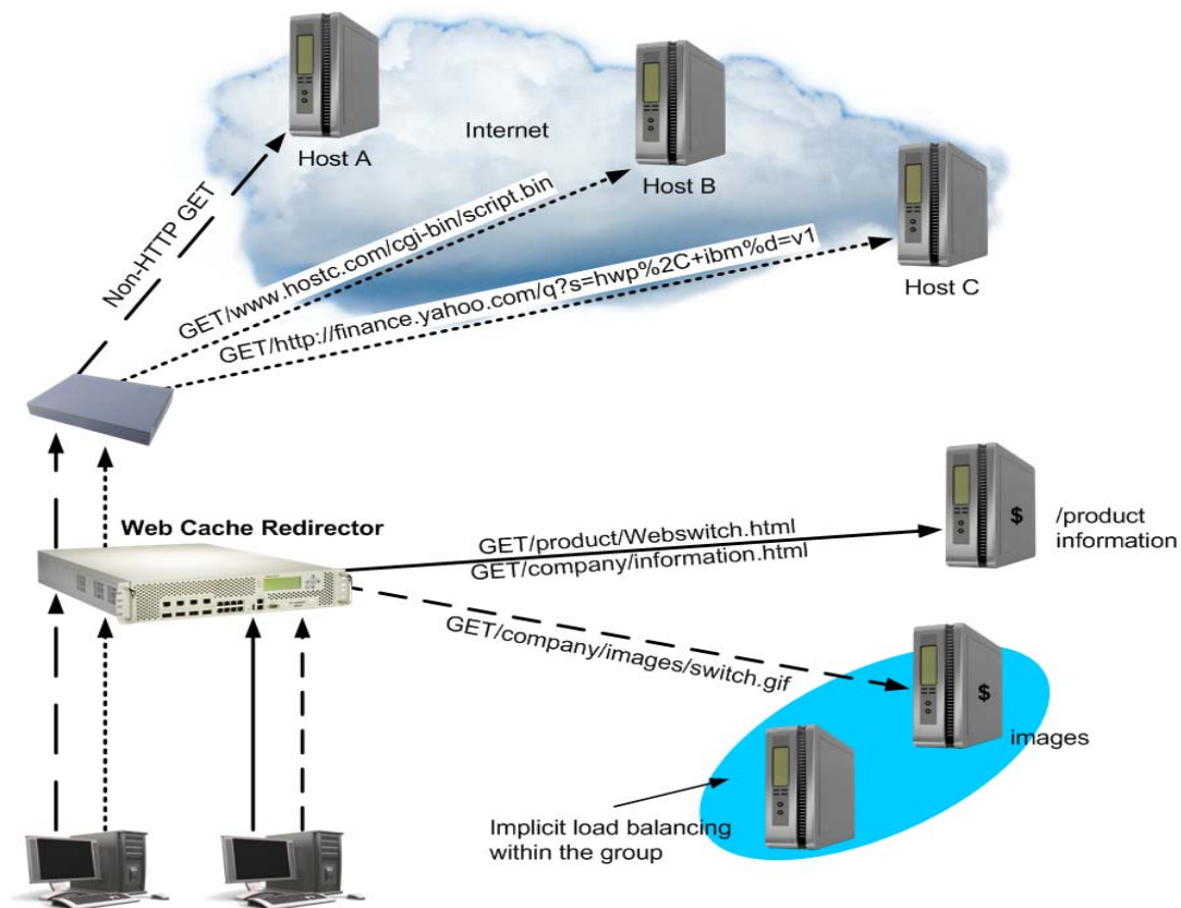
Figure 108: URL-Based Cache Redirection
