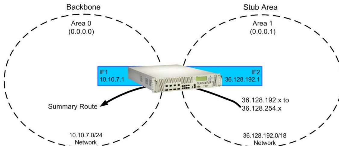
Figure 42: Summarizing Routes Example
