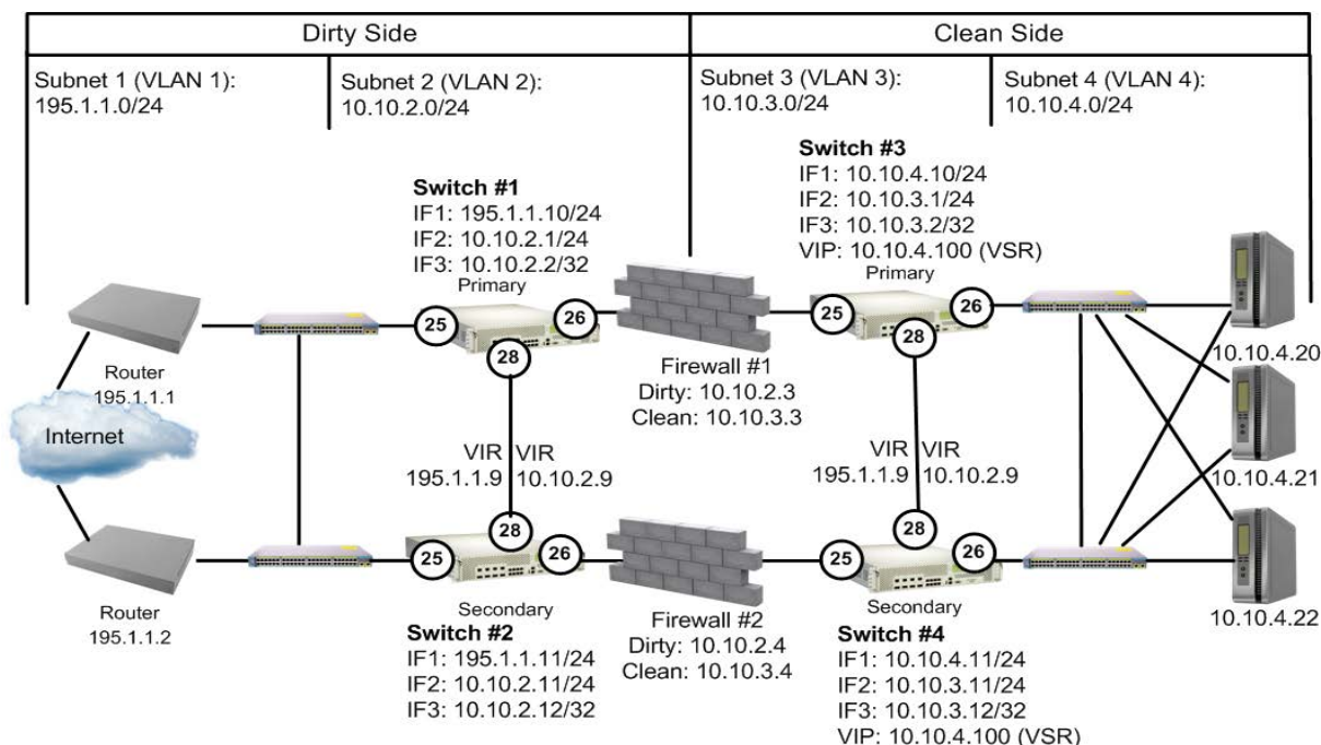
Figure 117: Example Four-Subnet FWLB Configuration
