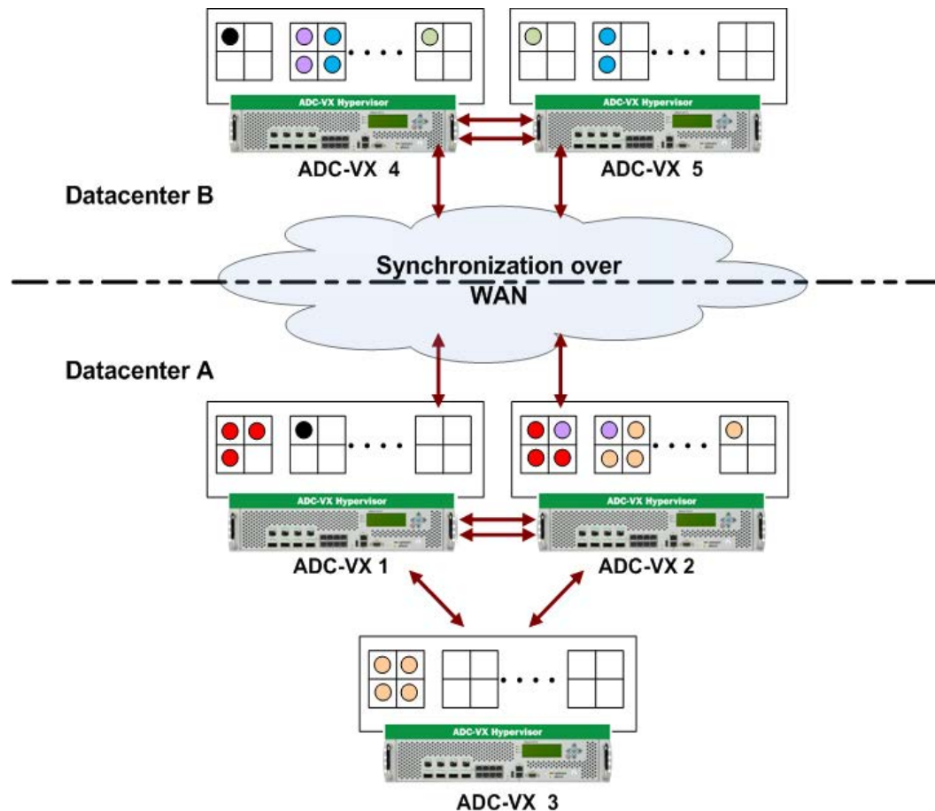
Figure 46: Example Peer Synchronization Topology
