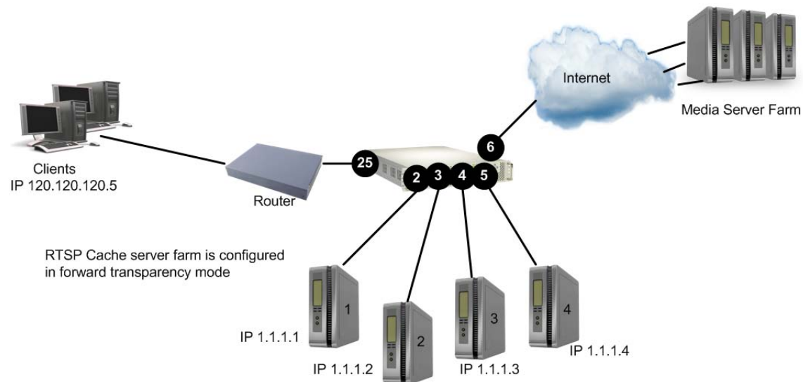
Figure 107: RTSP Cache Redirection Configuration
