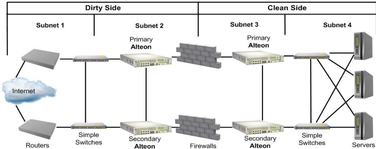
Figure 115: Four-Subnet FWLB Network Topology
