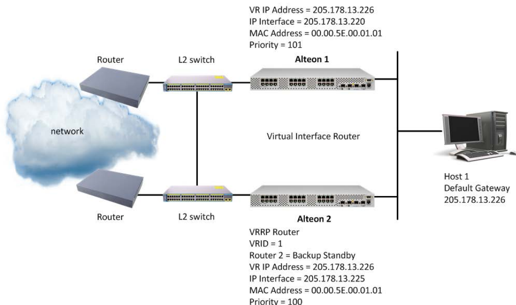
Figure 147: Virtual Interface Router Configuration
