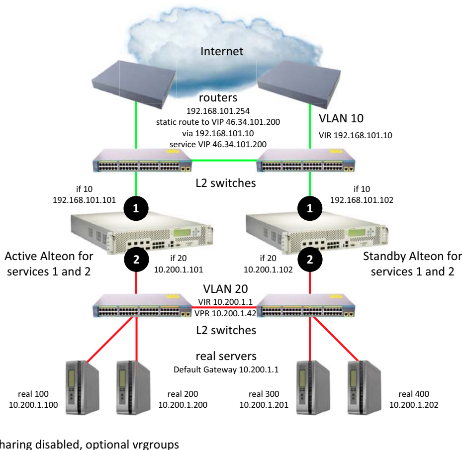
Figure 155: Separate Client and Server Ports with a Single Service, with PIP, and Dedicated VIP Subnet
