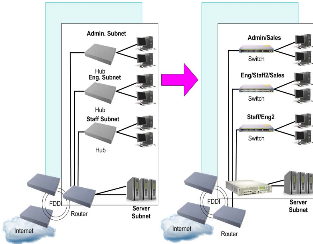
Figure 29: Example Topology Migration
