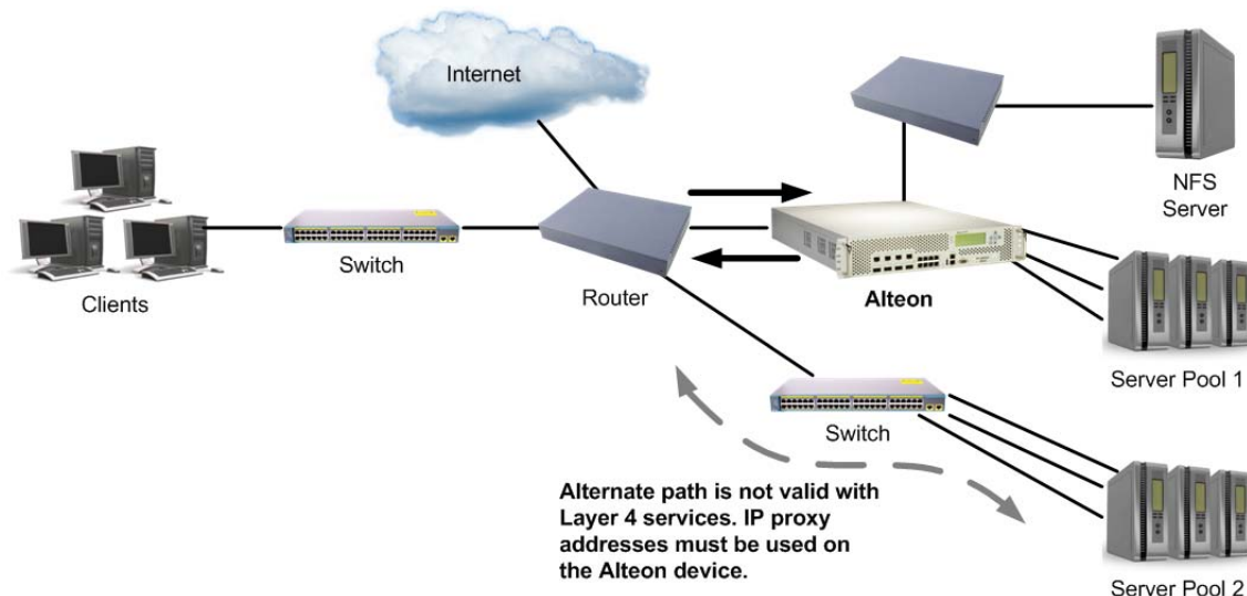
Figure 52: SLB Client/Server Traffic Routing
