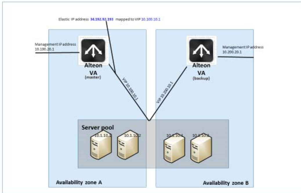
Figure 47: High Availability Initial Setup
