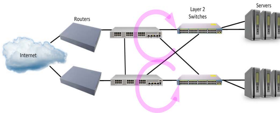
Figure 163: STP Resolving Cross-Redundancy Loops
