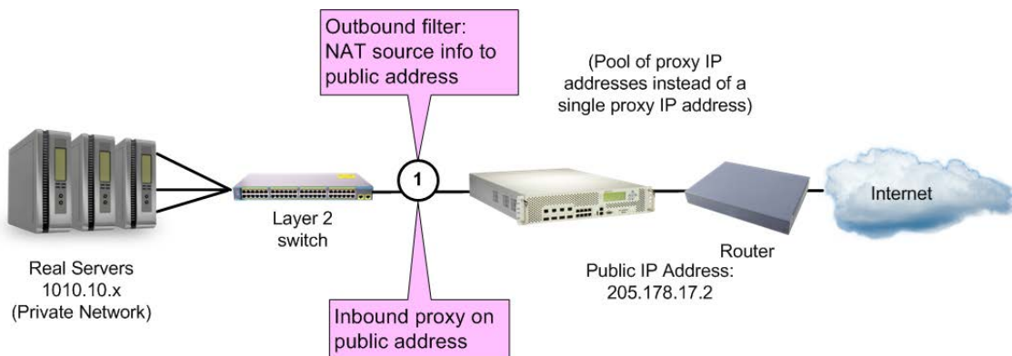
Figure 95: FTP Client NAT Example
