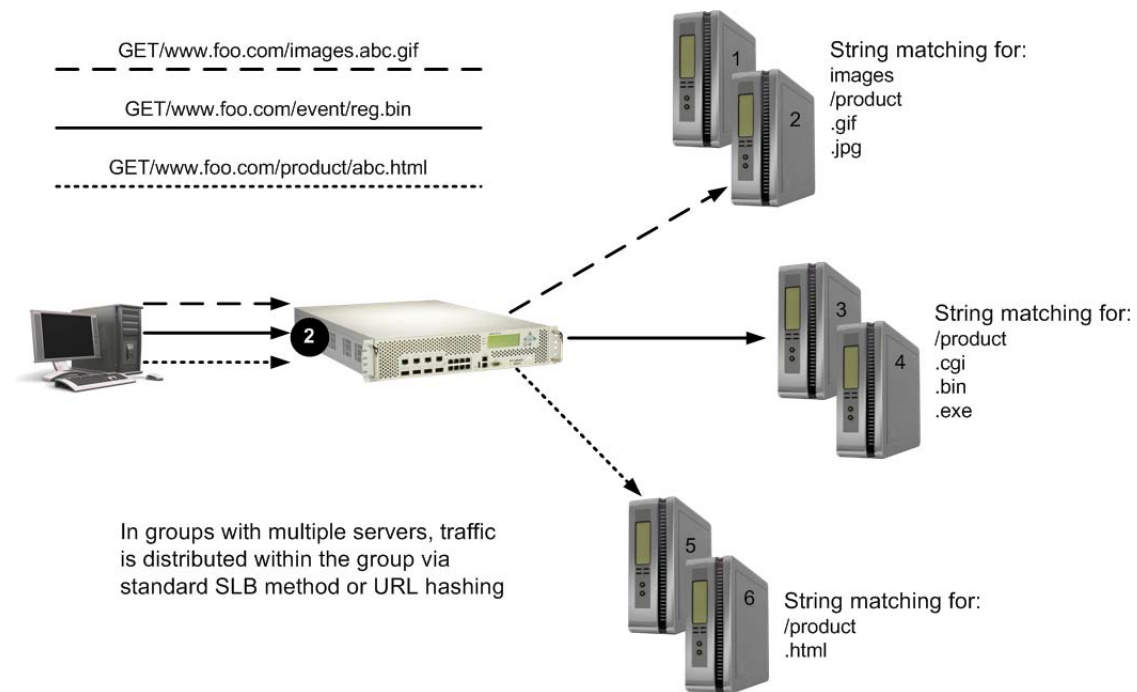
Figure 142: Requests with ".cgi" in the URL
