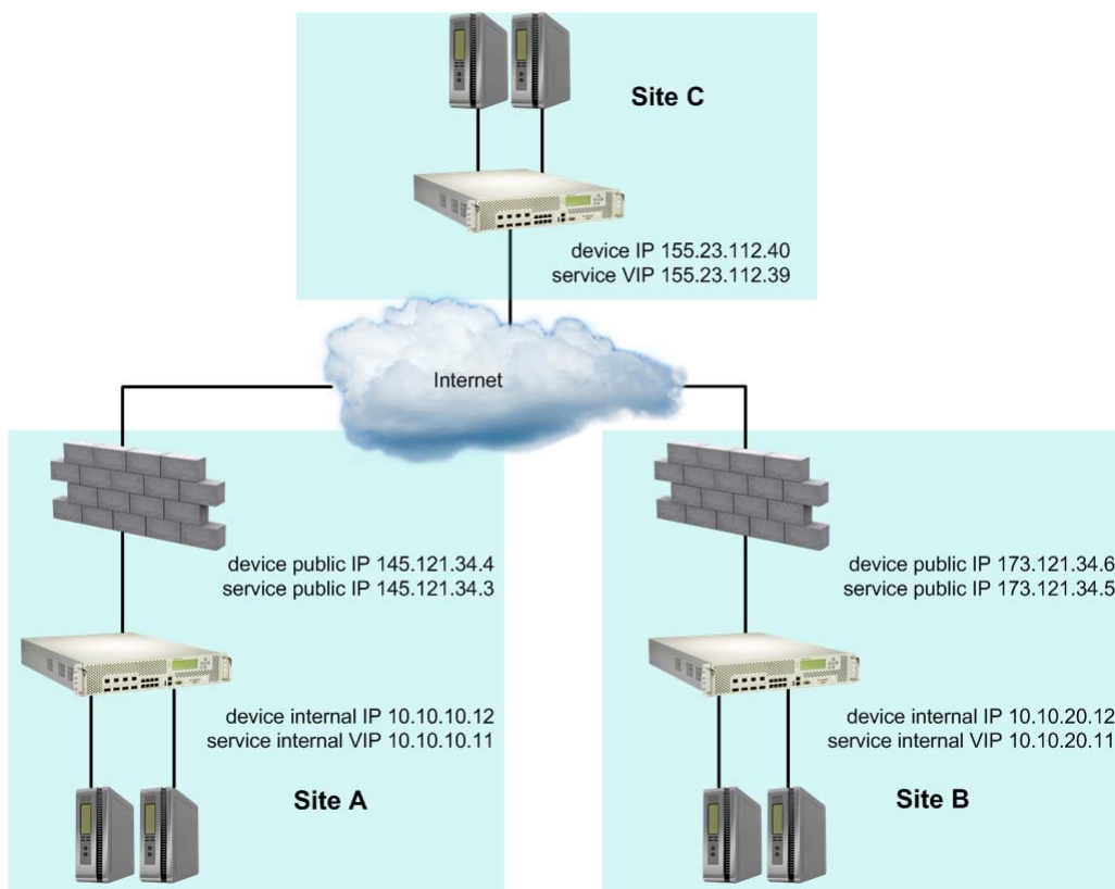
Figure 104: Network with GSLB Configuration Behind NAT Devices
