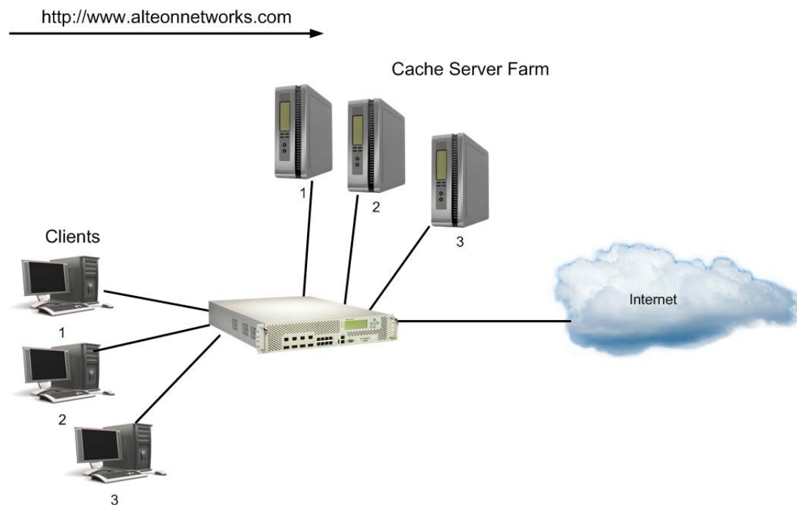
Figure 109: URL Hashing for Application Redirection
