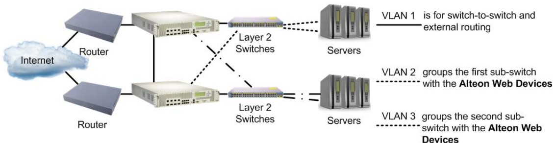
Figure 164: Using VLANs to Create Non-Looping Topologies
