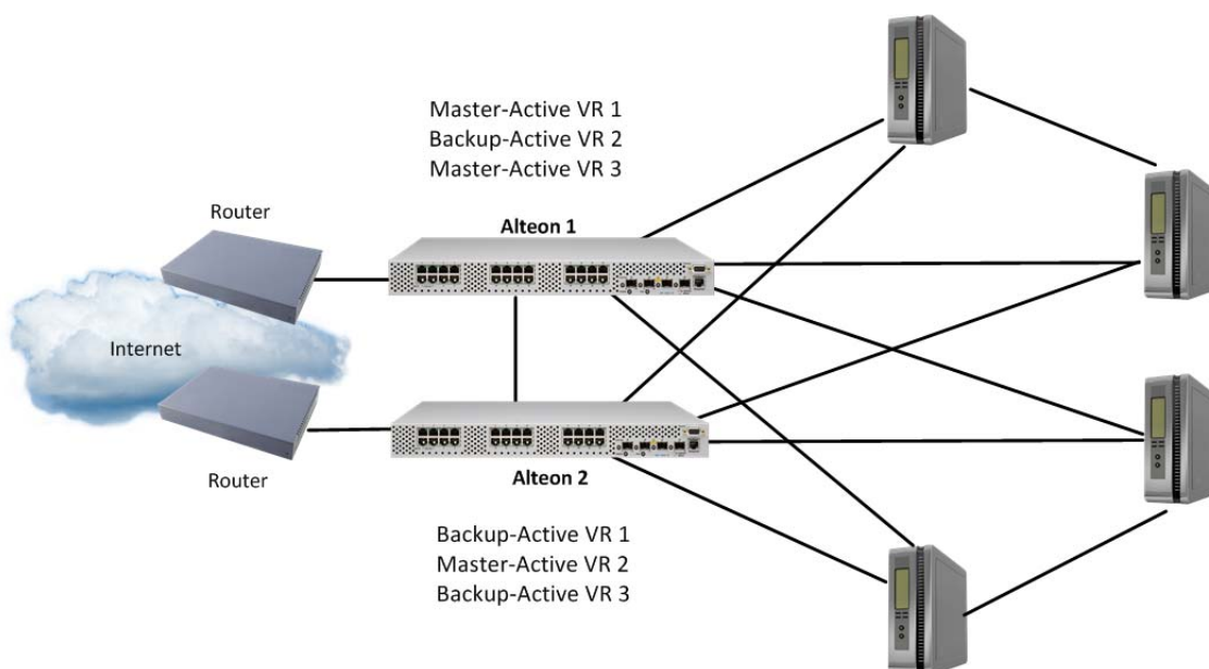
Figure 152: Active-Active Failover with Shared Interfaces
