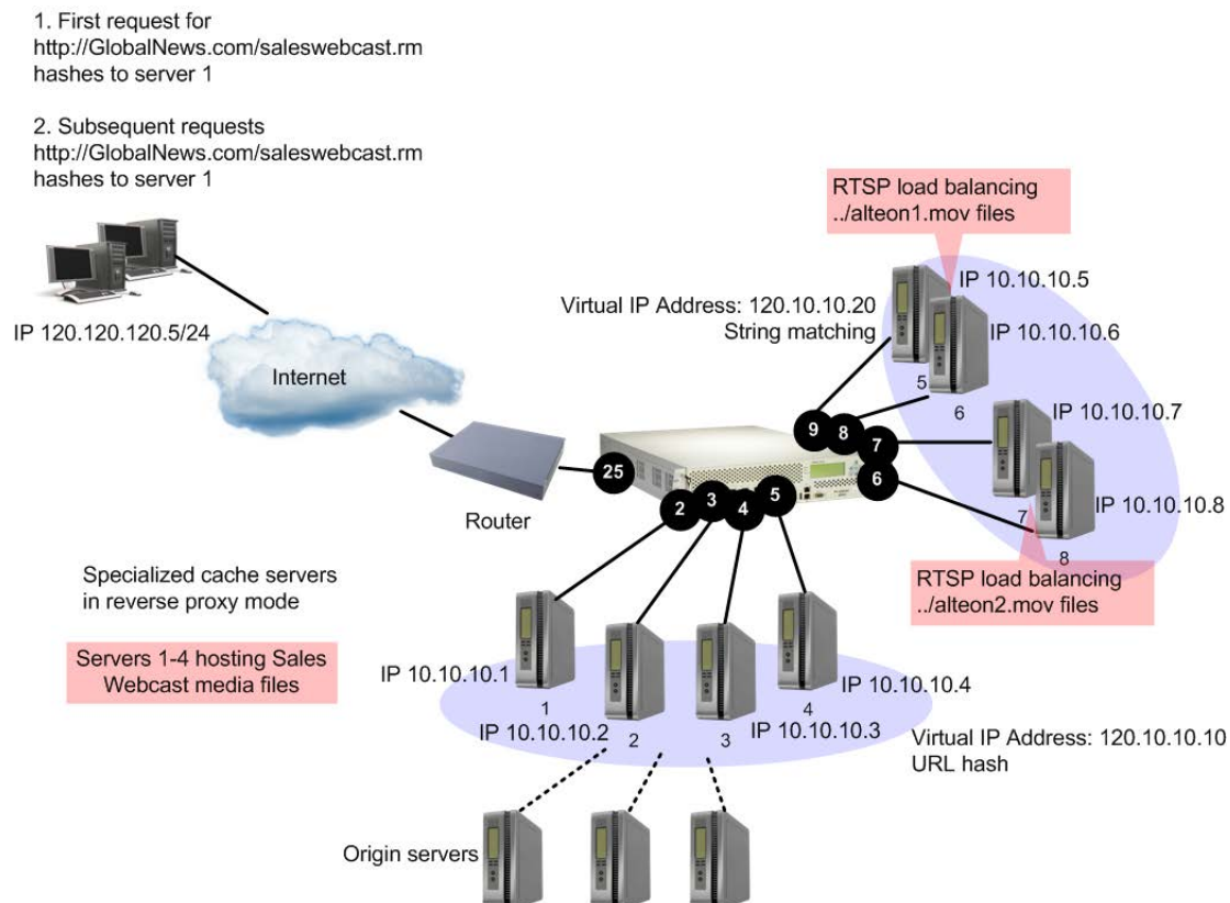
Figure 69: RTSP Load Balancing
