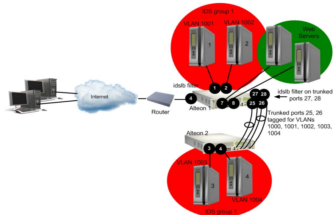
Figure 73: Server Load Balancing and IDS Load Balancing Across Multiple Alteon Platforms
