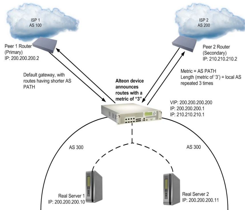
Figure 34: Example BGP Failover Configuration
