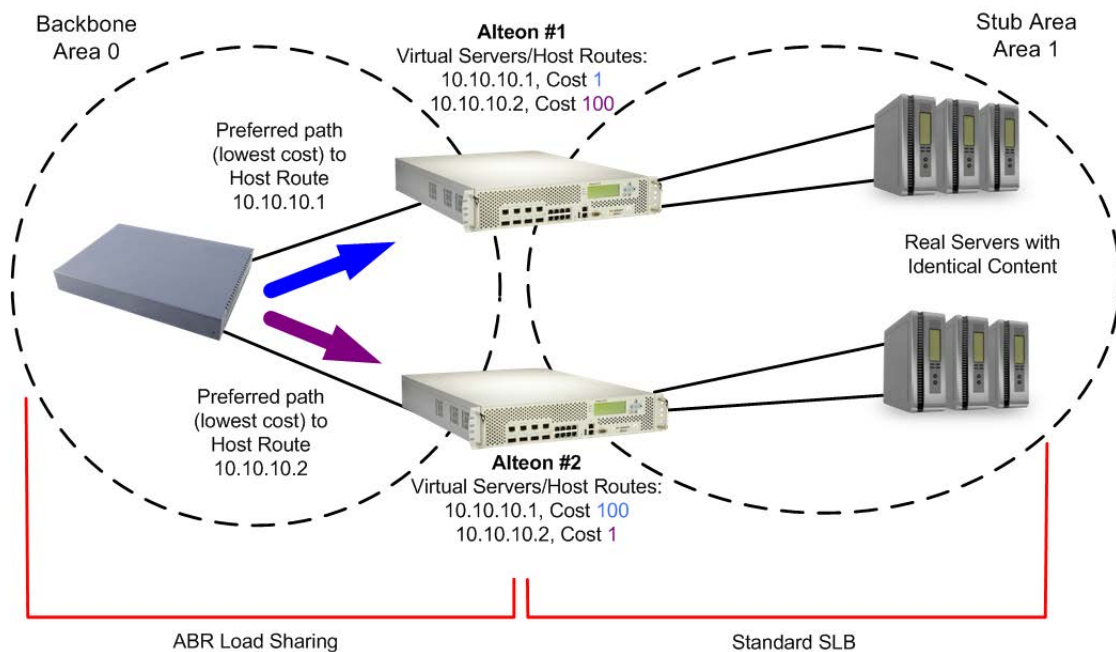
Figure 43: Host Routes Example
