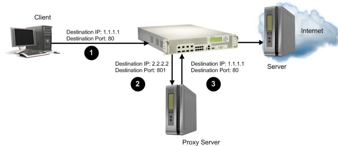
Figure 87: Redirecting Traffic with Port and IP Address Translation
