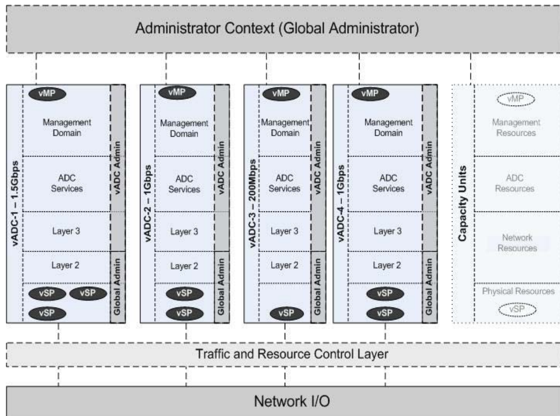
Figure 20: Network Architecture Configured to use ADC-VX
