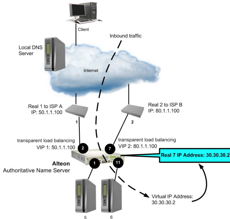
Figure 139: External Client Accessing Data from an SLB Group
