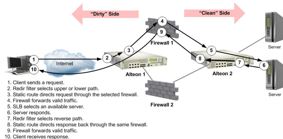
Figure 113: Basic FWLB Process
