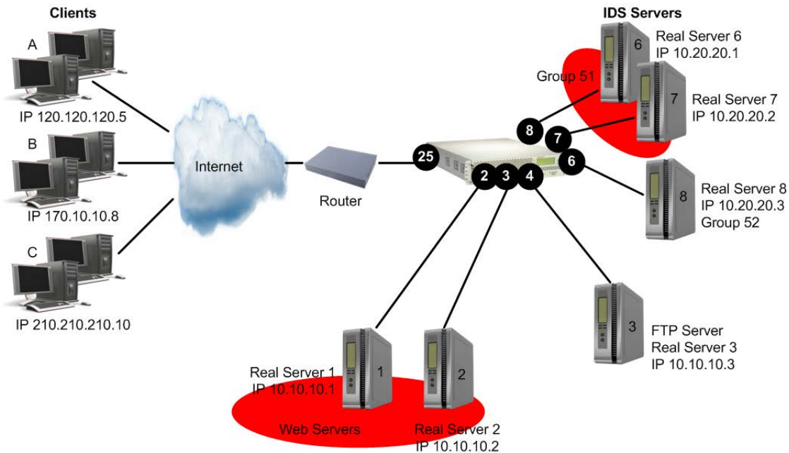
Figure 72: Server Load Balancing and IDS Load Balancing to Multiple Group
