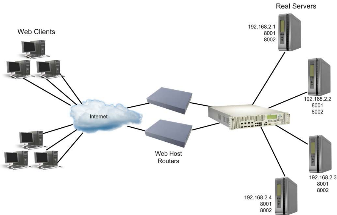
Figure 55: Basic Virtual Port-to-Real Port Mapping Configuration
