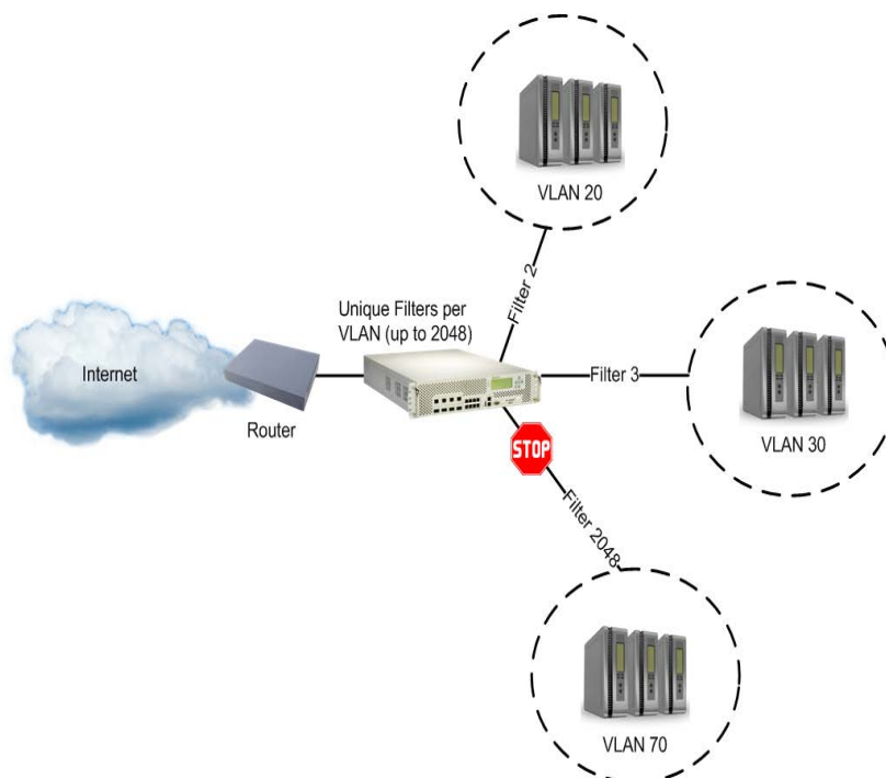
Figure 91: Example VLAN-Based Filtering Configuration
