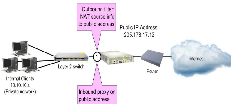
Figure 94: Dynamic NAT Example
