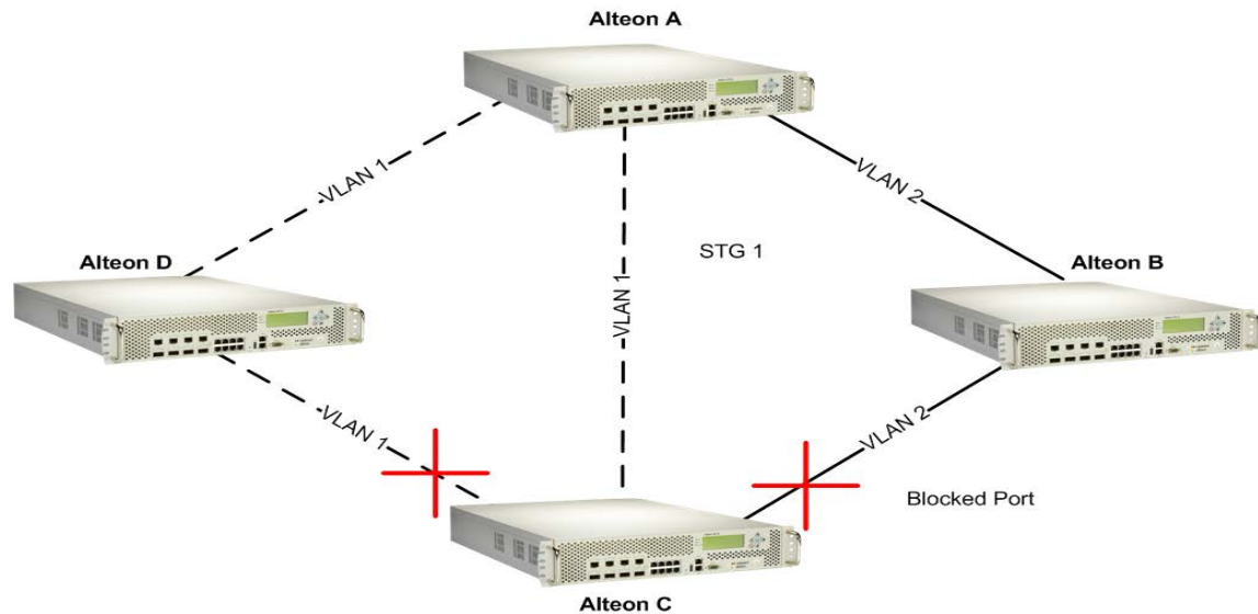
Figure 27: Four-Alteon Topology with a Single Spanning Tree
