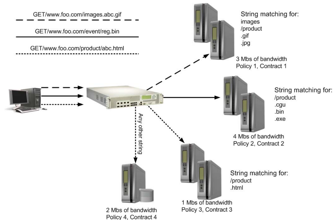
Figure 132: URL-Based SLB with Bandwidth Management
