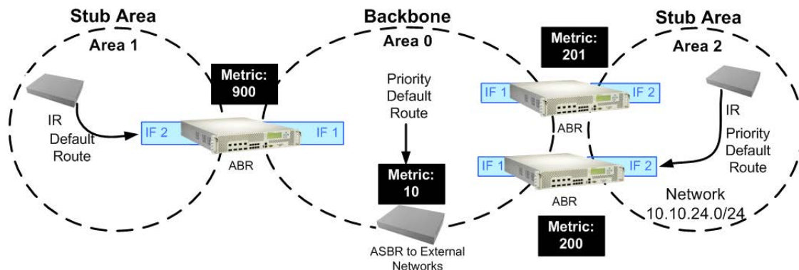
Figure 38: Default Routes Example
