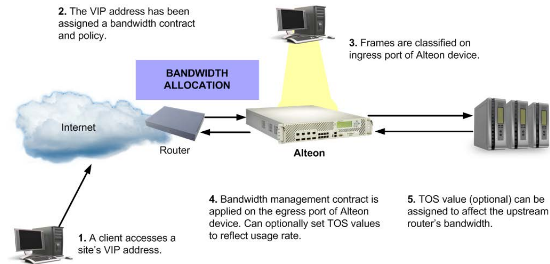
Figure 129: How Bandwidth Management Works
