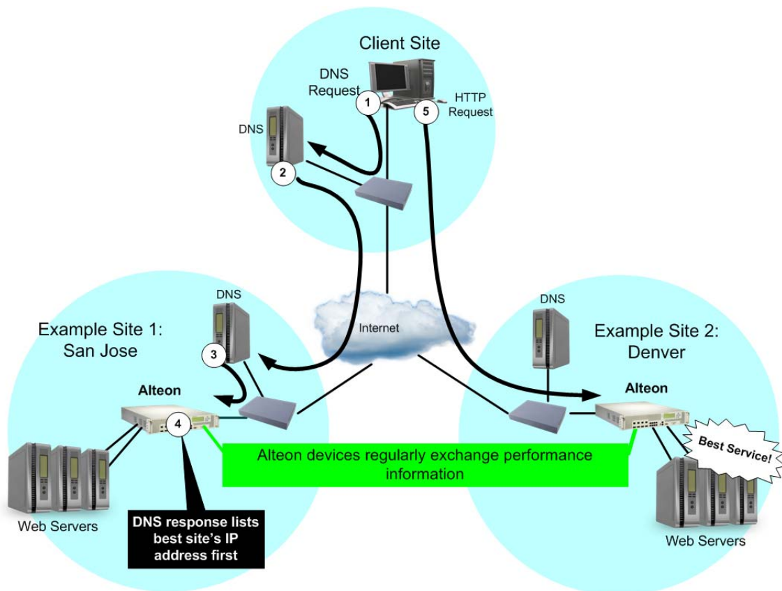
Figure 97: DNS Resolution with GSLB
