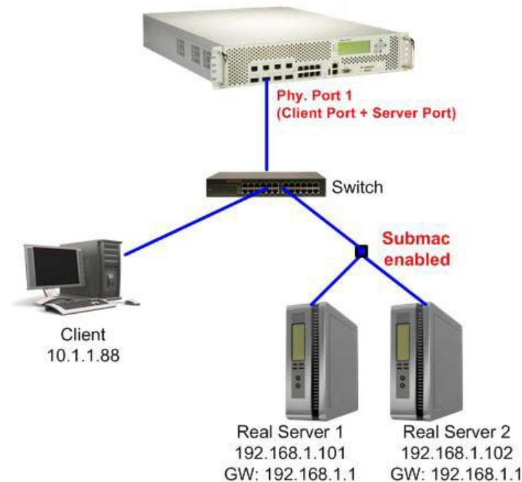
Figure 57: One Arm Topology
