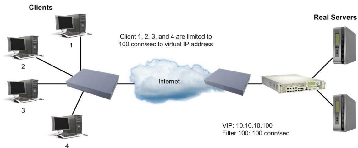
Figure 125: Limiting User Service to a Server
