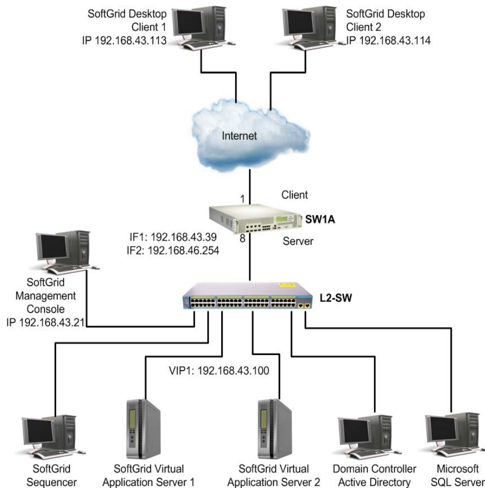
Figure 78: SoftGrid Load Balancing Network Topology
