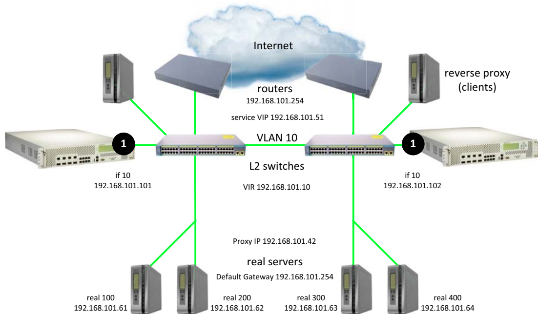
Figure 161: One Leg with PIP to Force Traffic Back to Source Alteon
