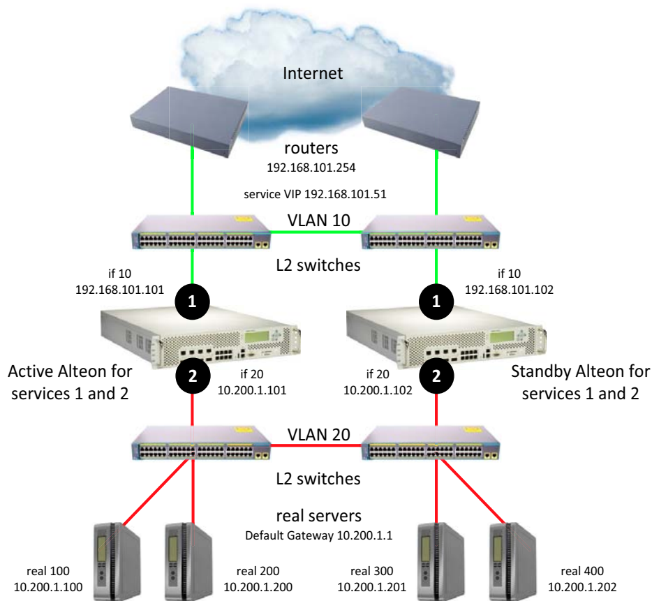
Figure 153: Multiple VLANs with Non-directly Attached Routers (Active-Standby)
