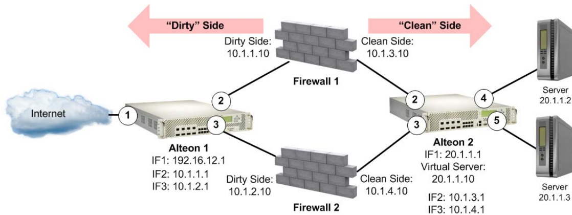
Figure 114: Basic FWLB Configuration Example
