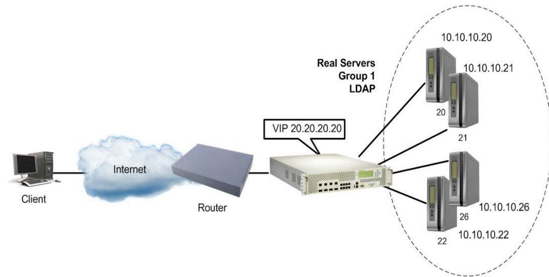
Figure 66: LDAP Load Balancing
