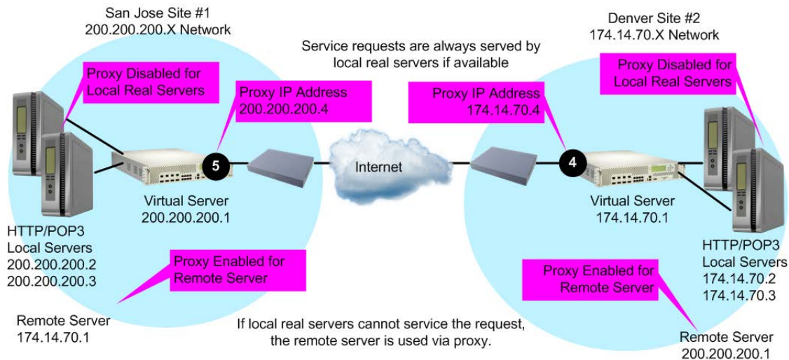
Figure 103: POP3 Request Fulfilled via Proxy IP
